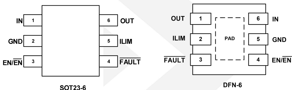
Figure 2. Pin assignment
