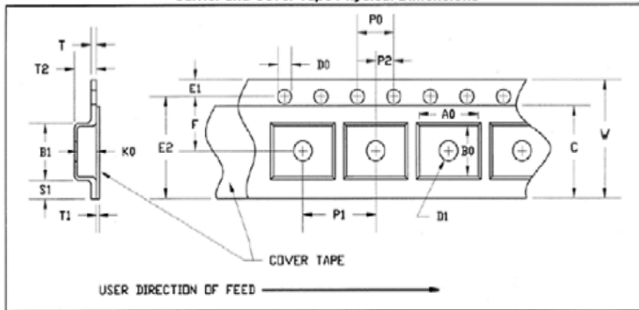
Carrier and Cover Tape Physical Dimensions
