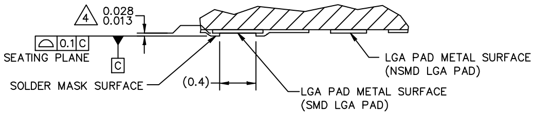
SECTION E-E 5
