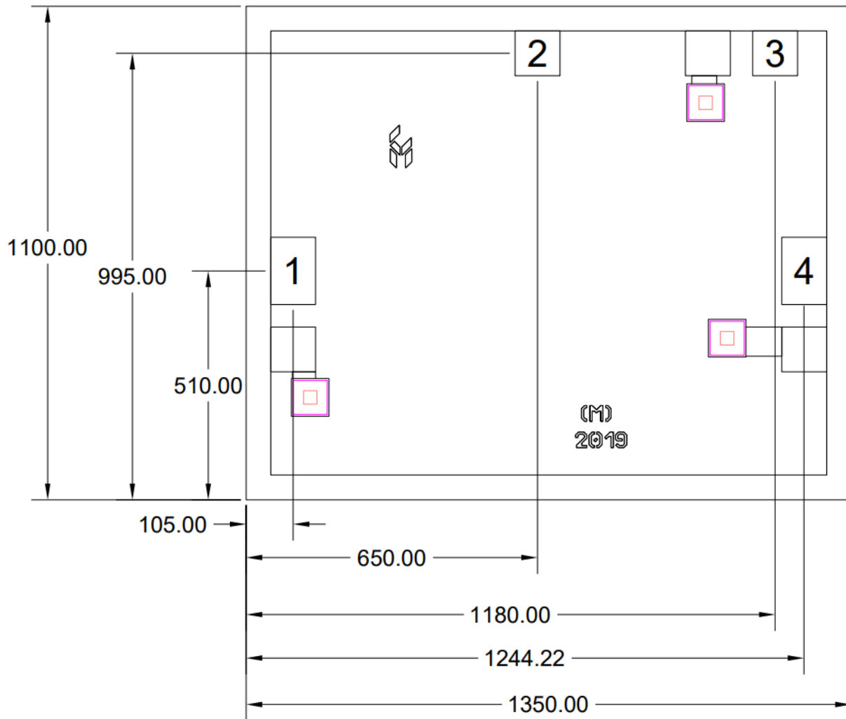
Die Outline (all dimensions in microns)
