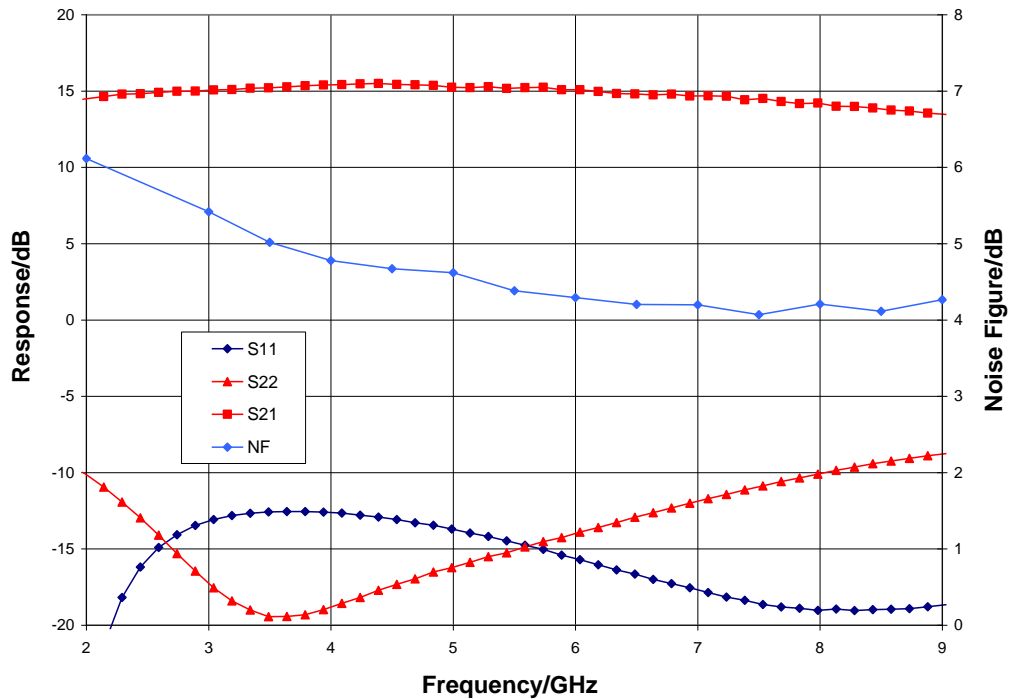
Narrow-band Performance, V_{dd} = 6.0\text{ V} , I_{dd} = 90\text{ mA} , T_A = 25\text{ °C}
