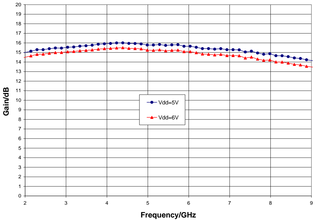
Gain vs. Supply Voltage, T_A = 25\text{ °C}
