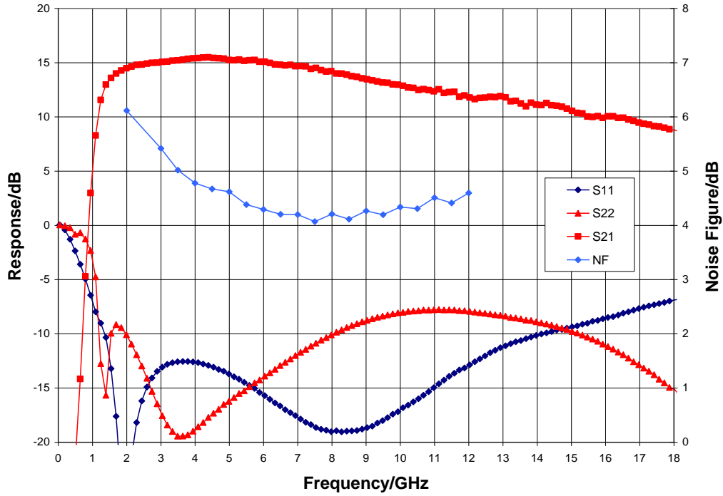
Broadband Performance, V_{dd} = 6.0\text{ V} , I_{dd} = 90\text{ mA} , T_A = 25\text{ °C}
