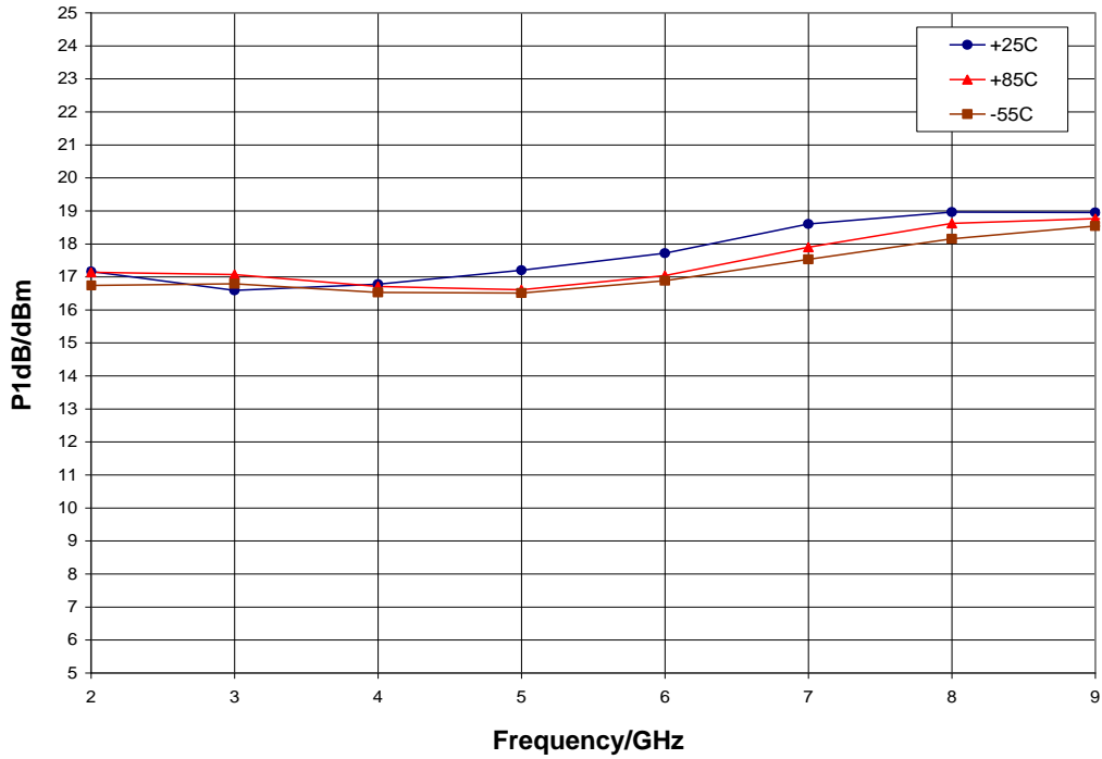
P1dB vs. Temperature, V_{dd} = 6.0\text{ V}
