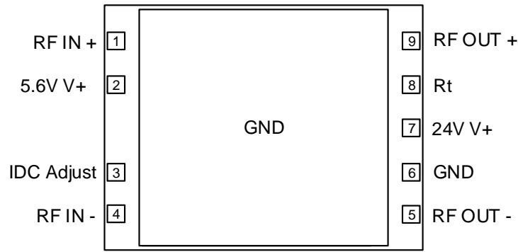
TOP PIN VIEW
