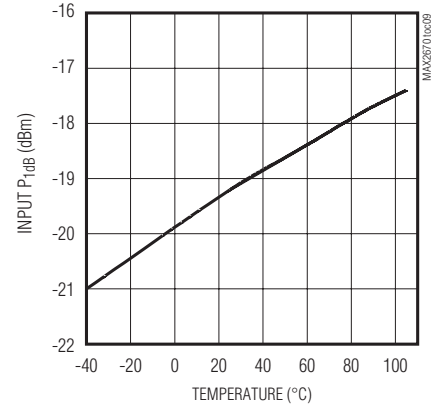
AMP 1 INPUT P 1dB vs. TEMPERATURE (WITH EXTERNAL INPUT IMPEDANCE MATCH)
