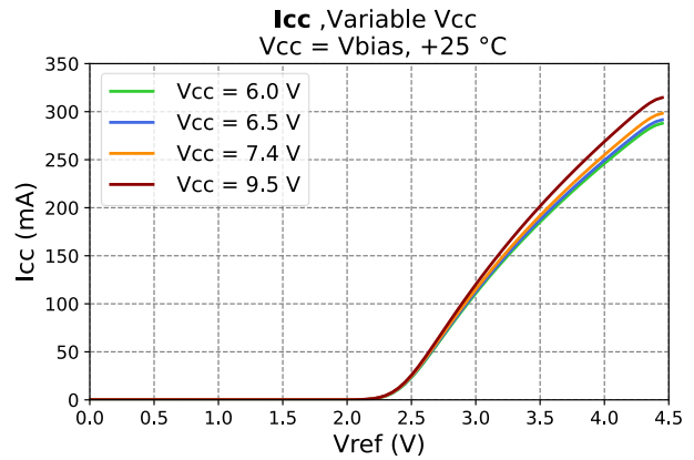
Figure 32 - Icc vs. Vref over Vcc
