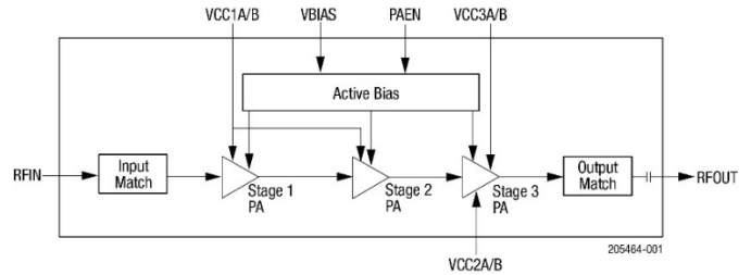
Figure 1. SKY66395-11 Block Diagram
