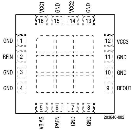
Figure 2. Pinout (Top View)
