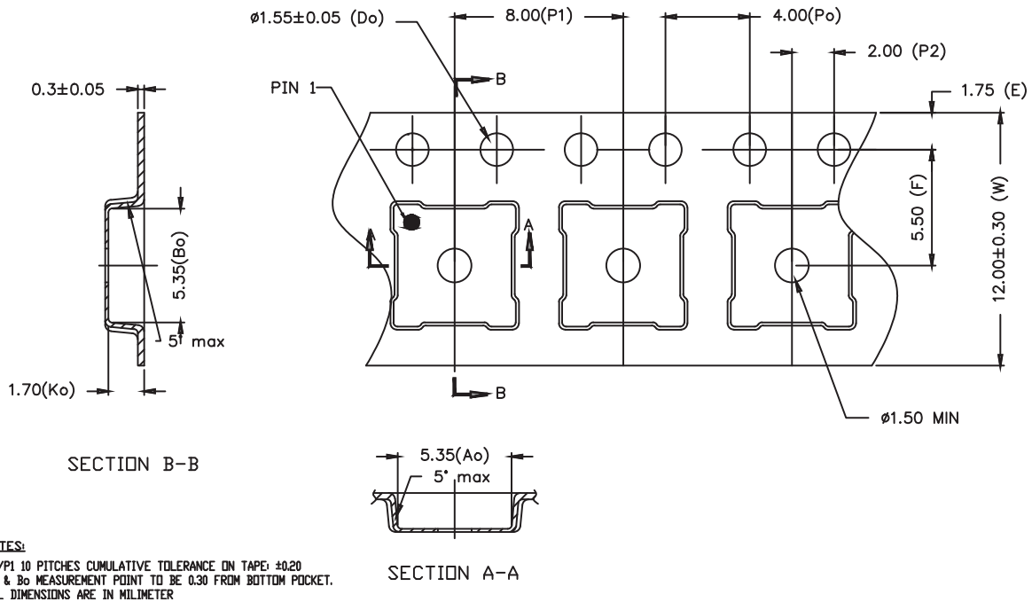
Figure 24. Tape and Reel Dimensions
