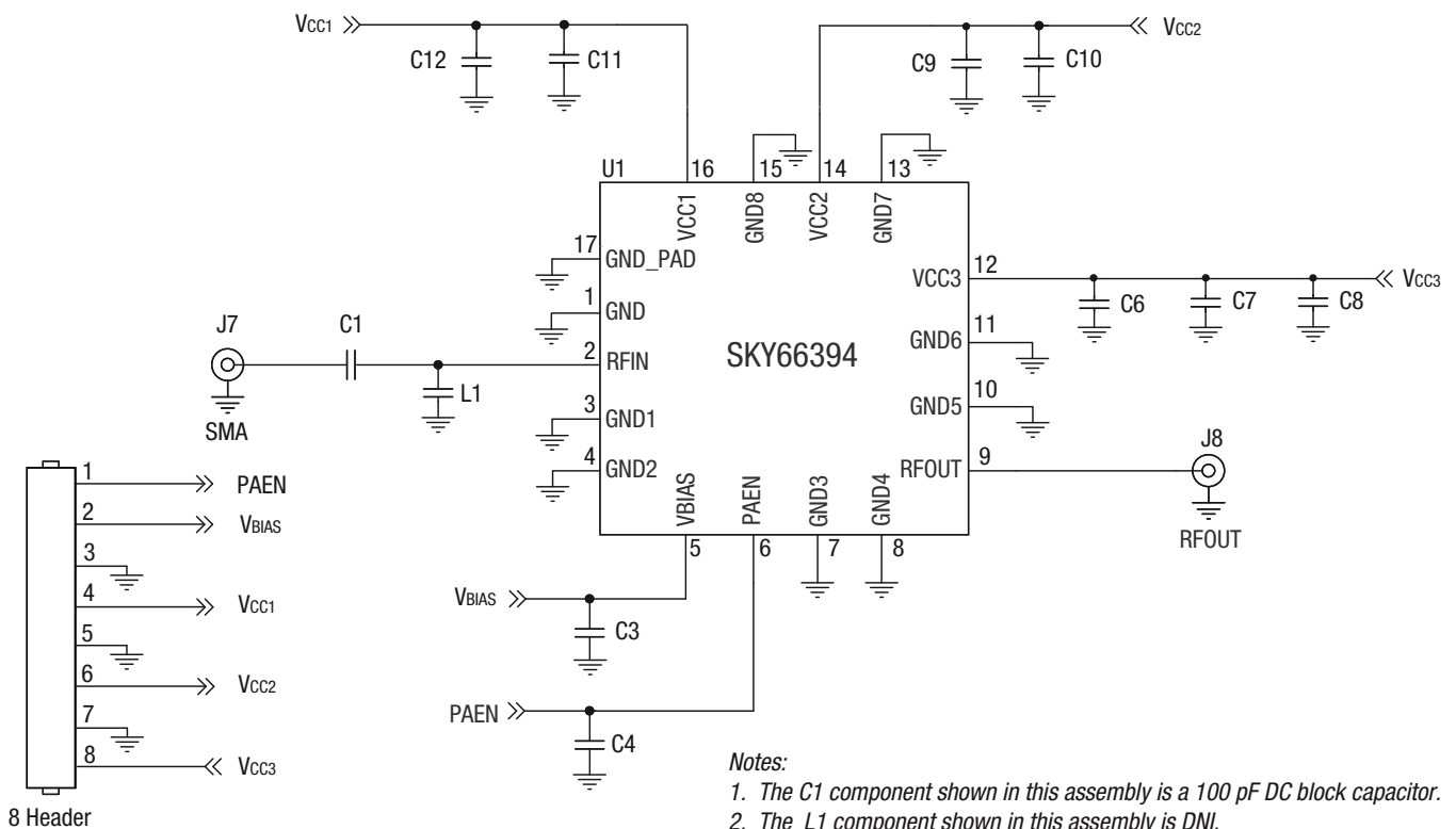
Figure 17. Application Schematic
