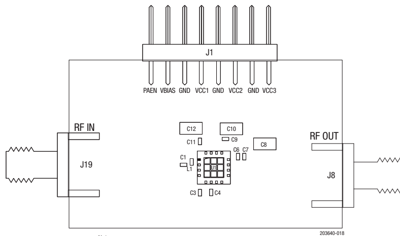
Figure 18. Evaluation Board Assembly Drawing
