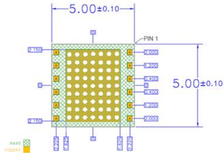
Recommended Via Pattern (63 Vias at 10mil Diameter)
