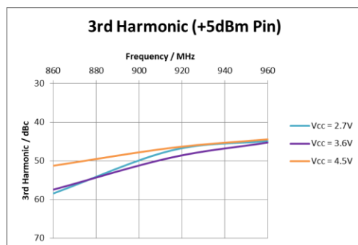
Figure 11: 3 rd Harmonic (+5 dBm Pin)
