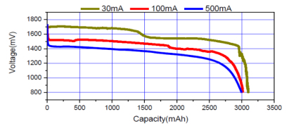
REMOTE RADIO 43ohm 4hrs/day 24ohm 15sec/min 8hrs
