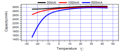
Discharge curve Constant current discharge
