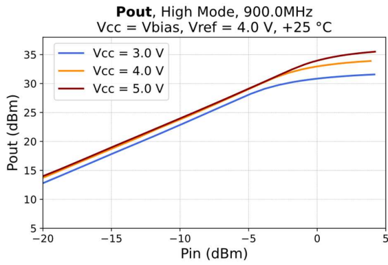
Figure 16 - Output Power vs. Input Power at 900 MHz
