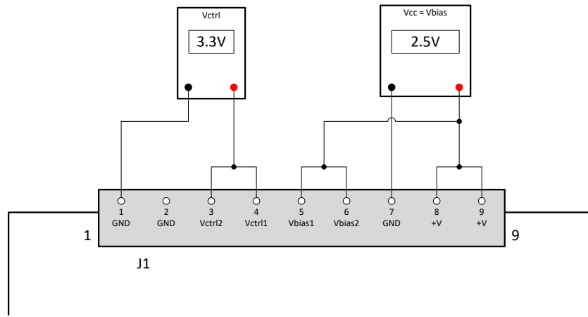
Figure 36: Alternative Power Supply Connections with Vbias = Vcc
