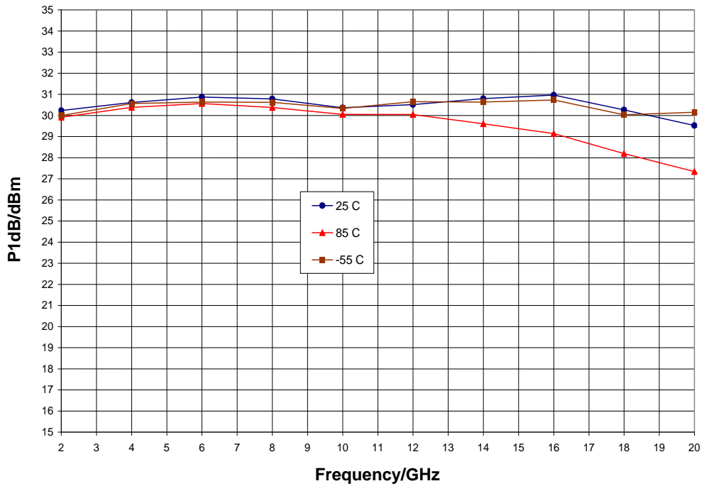
P1dB vs. Temperature, V_{dd} = 10\text{ V} , V_{gg} = -0.95\text{ V}
