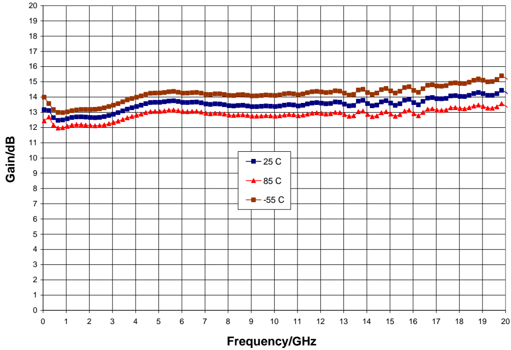
Gain vs. Temperature, V_{dd} = 10\text{ V} , V_{gg} = -0.95\text{ V}
