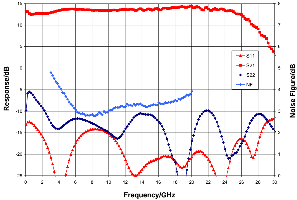
Broadband Performance, V_{dd} = 10\text{ V} , V_{gg} = -0.95\text{ V} , I_{dd} = 400\text{ mA} , T_A = 25\text{ °C}
