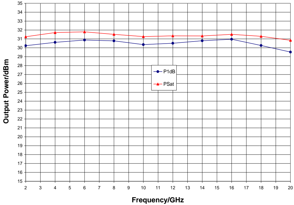
Output Power, V_{dd} = 10\text{ V} , V_{gg} = -0.95\text{ V} , T_A = 25\text{ }^\circ\text{C}
