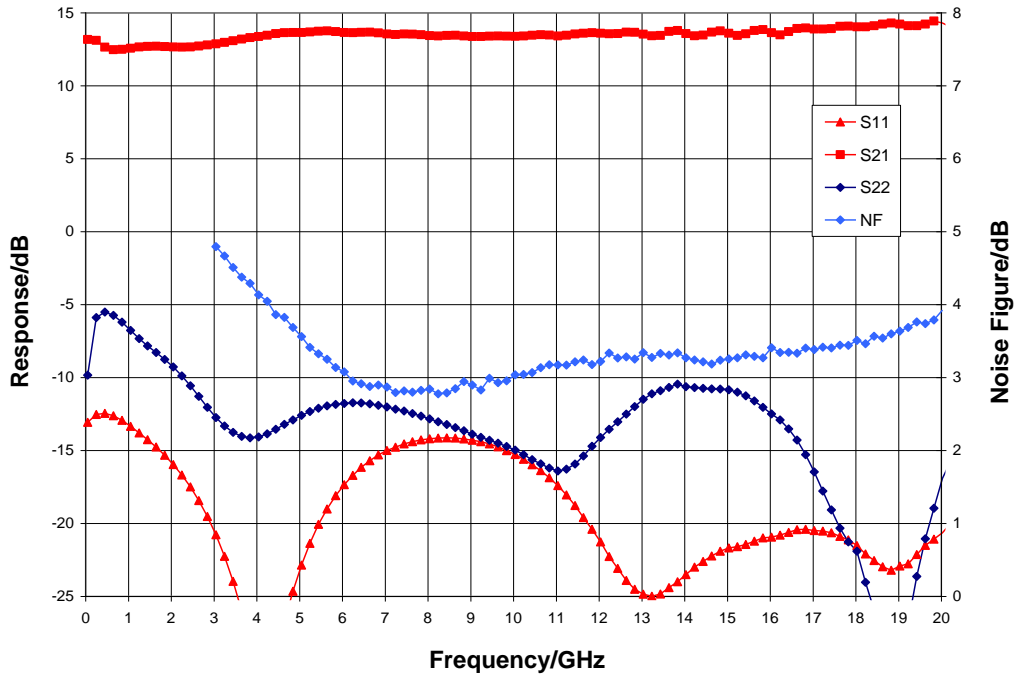
Narrow-band Performance, V_{dd} = 10\text{ V} , V_{gg} = -0.95\text{ V} , I_{dd} = 400\text{ mA} , T = 25\text{ °C}
