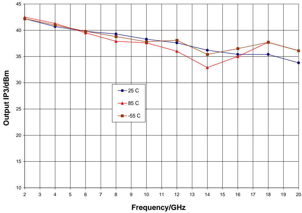
Output IP3 vs. Temperature, V_{dd} = 10\text{ V} , V_{gg} = -0.95\text{ V}
