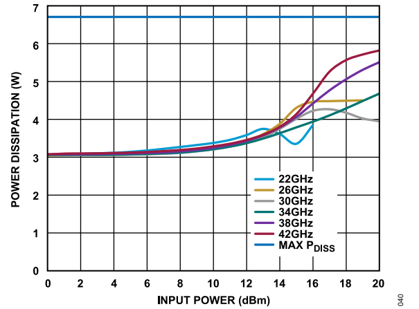
Figure 38. Power Dissipation vs. Input Power, T_A = 85^\circ\text{C}
