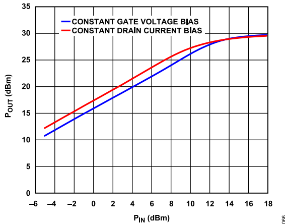
Figure 64. P_{OUT} vs. P_{IN} for Constant Gate Voltage Bias and Constant Drain Current Bias, V_{DD} = 5 V, Frequency = 32 GHz
