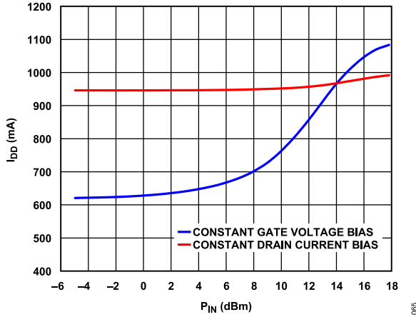
Figure 63. I_{DD} vs. Input Power ( P_{IN} ) for Constant Gate Voltage Bias and Constant Drain Current Bias, V_{DD} = 5 V, Frequency = 32 GHz
