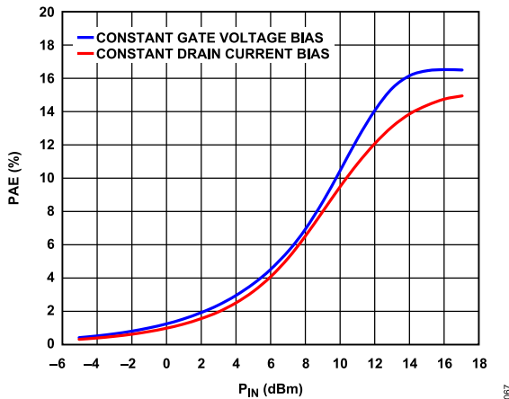
Figure 65. PAE vs. P_{IN} for Constant Gate Voltage Bias and Constant Drain Current Bias, V_{DD} = 5 V, Frequency = 32 GHz
