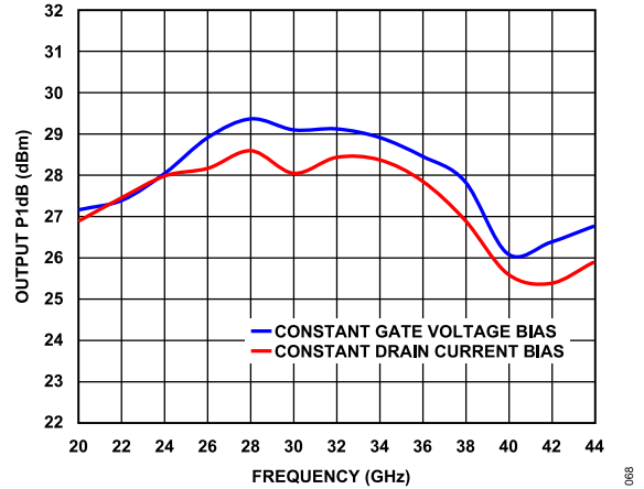
Figure 66. Output P1dB vs. Frequency for Constant Gate Voltage Bias and Constant Drain Current Bias, V_{DD} = 5 V
