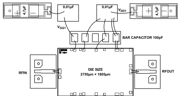
Figure 57. Alternate Assembly Diagram
