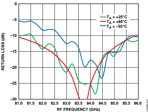
Figure 21. RF Return Loss vs. RF Frequency at Various Temperatures, RFIN = -10 dBm, LO = 2 dBm at 12 GHz
