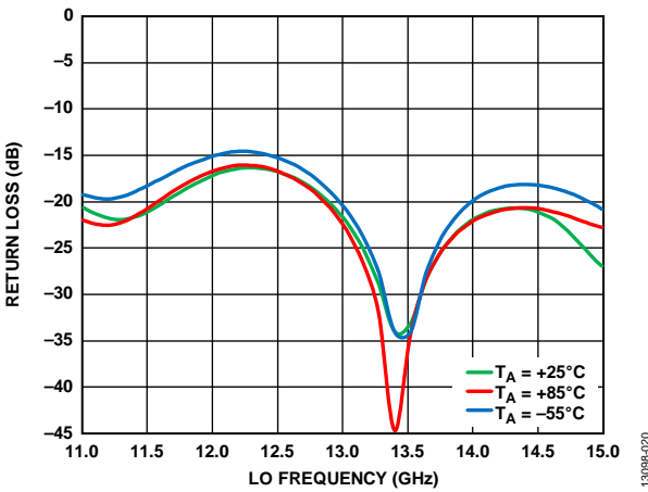
Figure 20. LO Return Loss vs. LO Frequency at Various Temperatures, LO = 2 dBm
