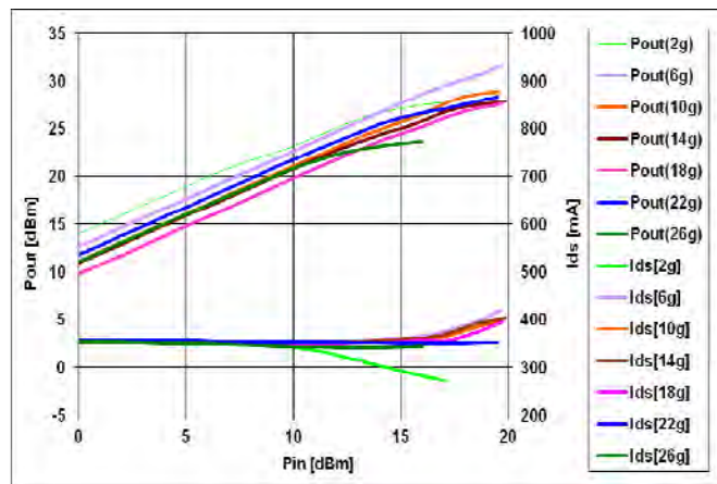
Pout and Ids vs. Pin
