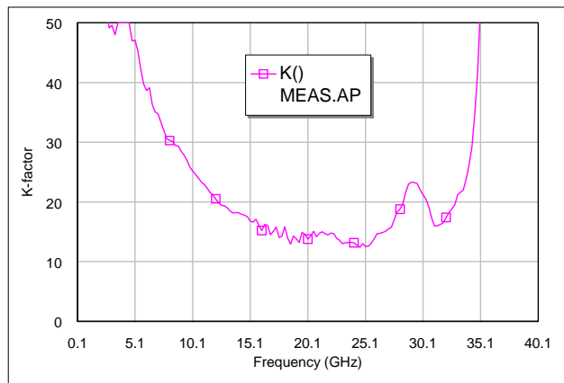
K-factor vs. Frequency
