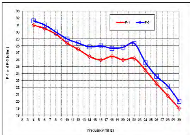
P-1 and P-3 vs. Frequency
