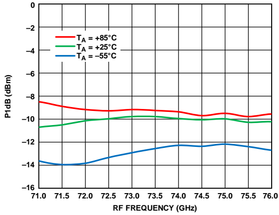
Figure 164. Input P1dB vs. RF Frequency at Various Temperatures, LO = 2 dBm, IF = 1000 MHz, V_{DLNA} = 4\text{ V}
