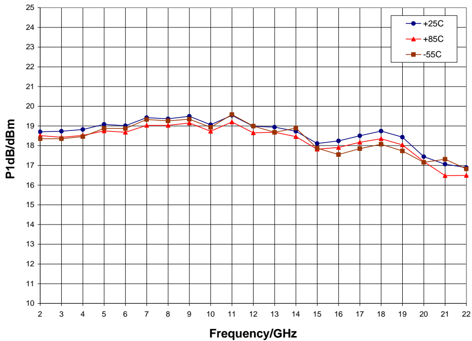
P1dB vs. Temperature, V_{dd} = 5\text{ V} , V_{gg} = -0.6\text{ V}
