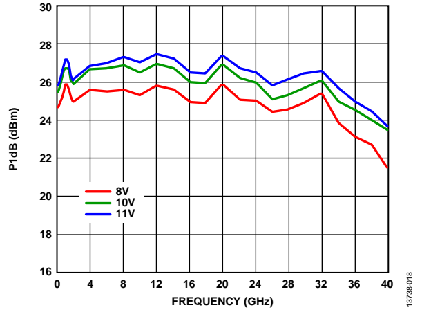
Figure 18. P1dB vs. Frequency for Various Supply Voltages
