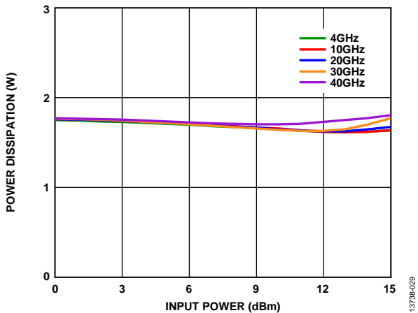
Figure 29. Power Dissipation
