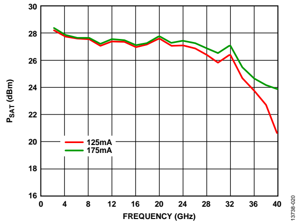
Figure 20. PSAT vs. Frequency and Supply Current
