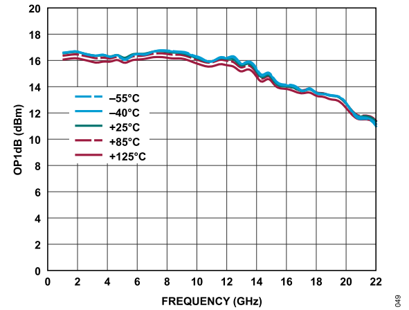
Figure 49. OP1dB vs. Frequency for Various Temperatures, 1 GHz to 22 GHz, V_{DD} = 3.3 V, I_{DQ} = 55 mA, R_{BIAS} = 542 Ω
