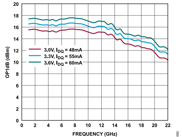
Figure 50. OP1dB vs. Frequency for Various Supply Voltages and I_{DQ} Values, 1 GHz to 22 GHz, R_{BIAS} = 542 Ω
