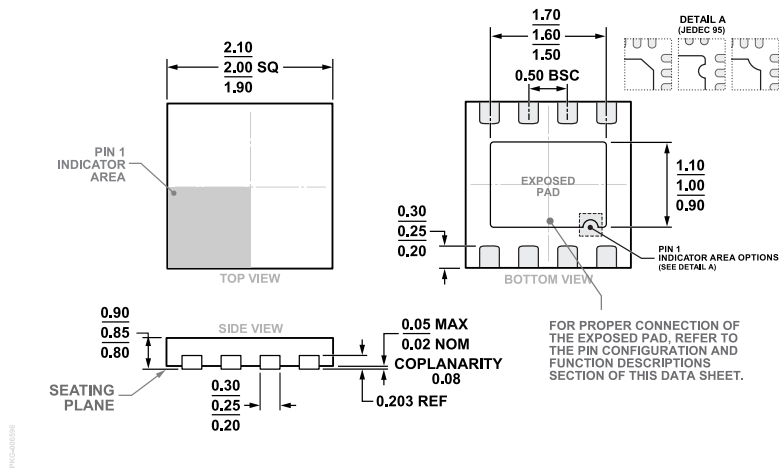
Figure 116. 8-Lead Lead Frame Chip Scale Package [LFCSP] 2 mm × 2 mm Body and 0.85 mm Package Height (CP-8-30) Dimensions shown in millimeters
