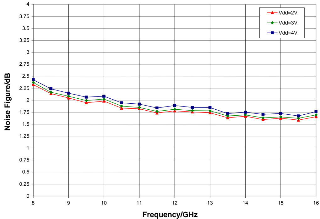
Noise Figure vs. V_{dd} , T_A = 25\text{ }^\circ\text{C}
