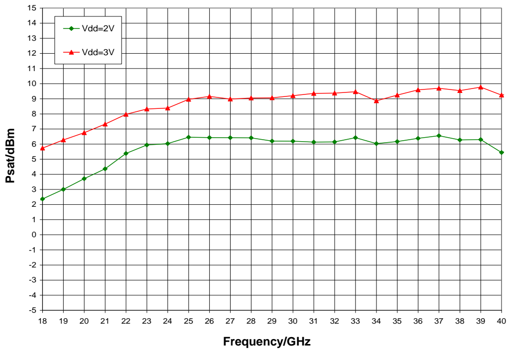
Psat vs. V_{dd} , V_{gg} = 3.0\text{ V} , T_A = 25\text{ }^\circ\text{C}
