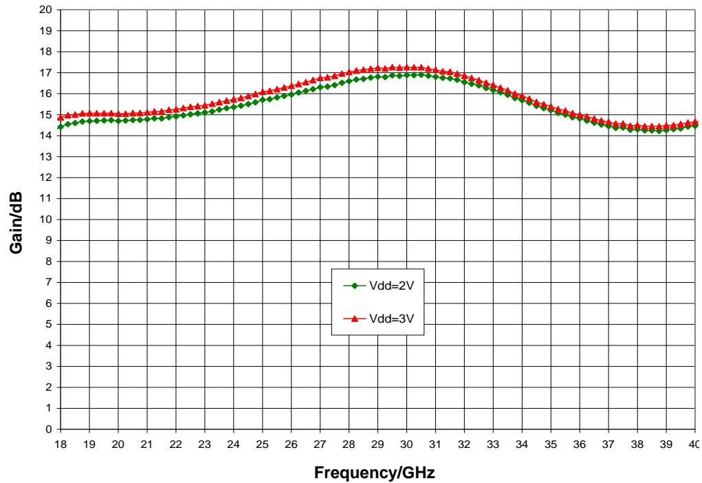
Gain vs. V_{dd} , V_{gg} = 3.0\text{ V} , T_A = 25\text{ °C}
