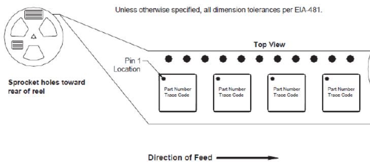
Figure 1: 5.000 mm x 5.000 mm (Carrier Tape Drawing with Part Orientation)
