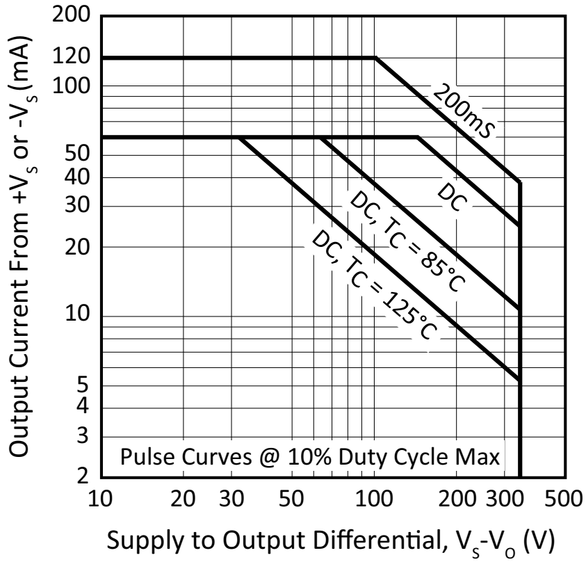
Figure 17: PA341DW SOA
