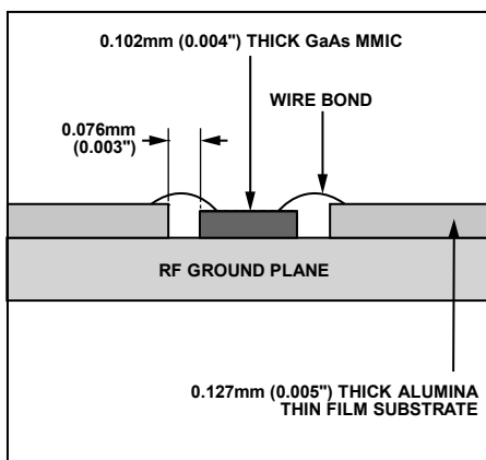
Figure 48. Die Without the Moly Tab
