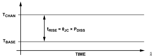
Figure 48. Channel Temperature Rise for Continuous Bias Condition
