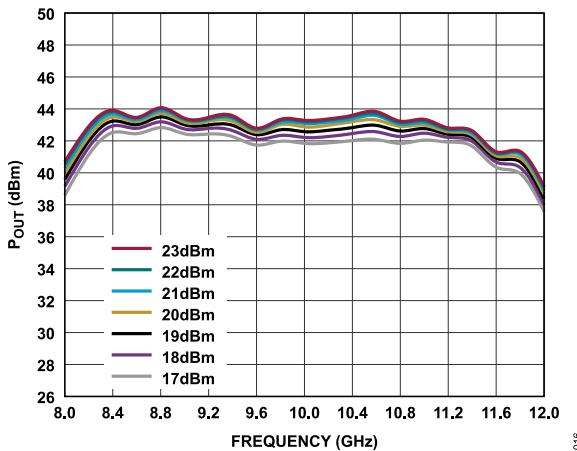
Figure 18. P_{OUT} vs. Frequency for Various P_{IN} Levels
