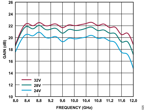
Figure 19. Gain at P_{IN} = 22 dBm vs. Frequency for Various Supply Voltages at I_{DQ} = 200 mA
