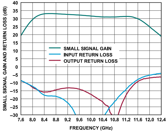
Figure 10. Small Signal Gain and Return Loss vs. Frequency
