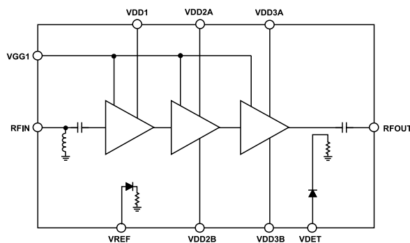
Figure 46. Basic Block Diagram
