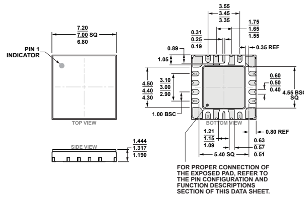
Figure 50. 18-Terminal Ceramic Leadless Chip Carrier with Heat Sink [LCC_HS] (EH-18-1) Dimensions shown in millimeters
