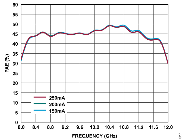
Figure 27. PAE at P_{IN} = 22 dBm vs. Frequency for Various I_{DQ} Values at V_{DD} = 28 V
