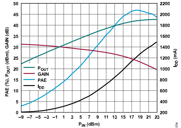
Figure 33. P_{OUT} , Gain, PAE, and I_{DD} vs. P_{IN} at 11.4 GHz
