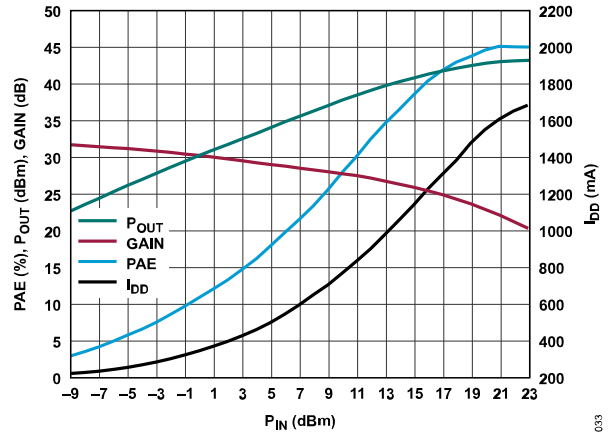
Figure 32. P_{OUT} , Gain, PAE, and I_{DD} vs. P_{IN} at 10.0 GHz
