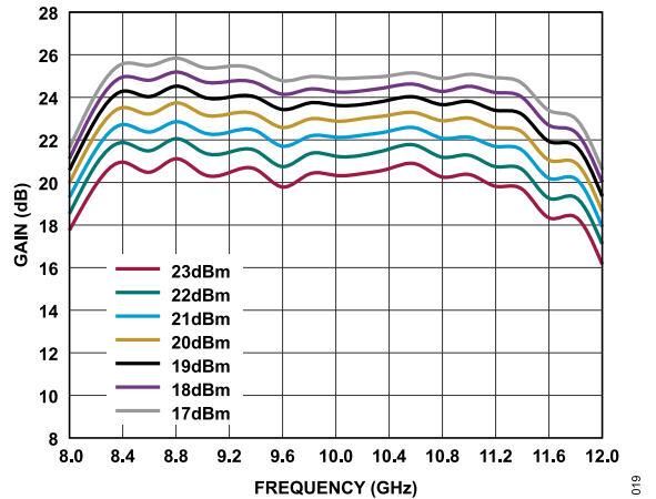
Figure 20. Gain vs. Frequency for Various P_{IN} Levels
