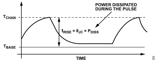
Figure 49. Pulsed Bias at Low Duty Cycle
