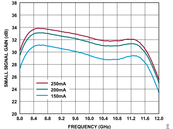
Figure 15. Small Signal Gain vs. Frequency for Various I_{DQ} Values at V_{DD} = 28 \text{ V}
