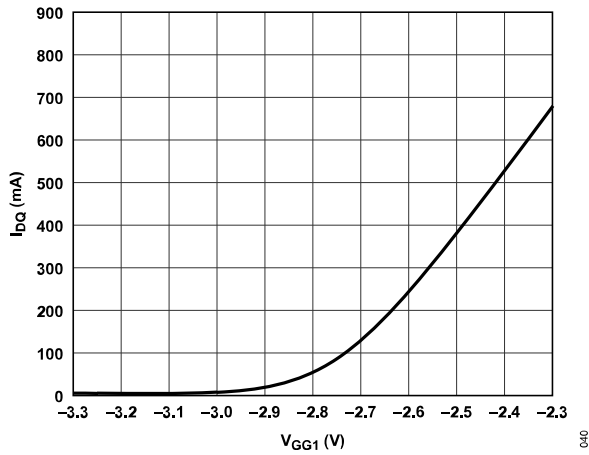
Figure 29. I_{DQ} vs. V_{GG1} , V_{DD} = 28 V
