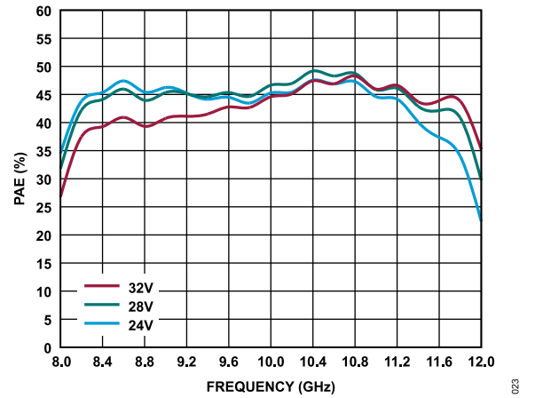
Figure 26. PAE at P_{IN} = 22 dBm vs. Frequency for Various Supply Voltages at I_{DQ} = 200 mA
