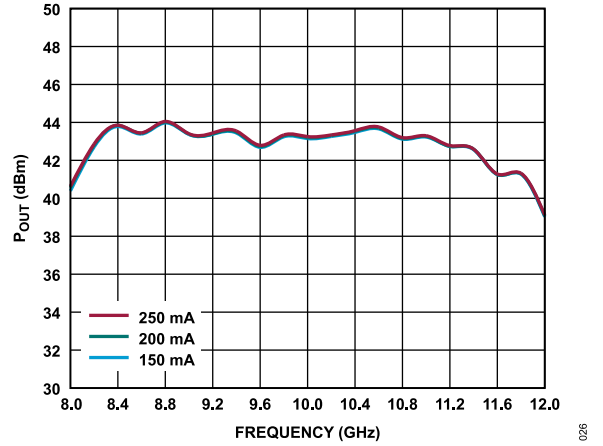
Figure 25. P_{OUT} at P_{IN} = 22 dBm vs. Frequency for Various I_{DQ} Values at V_{DD} = 28 V
