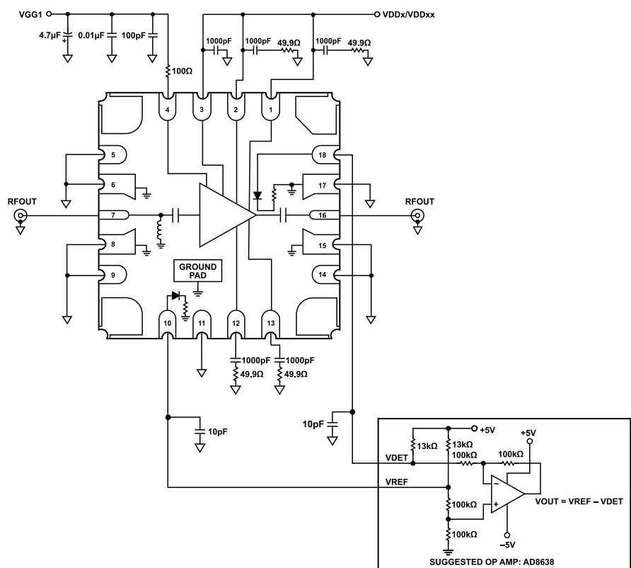
Figure 47. Basic Connections
