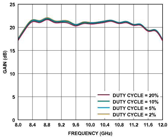
Figure 41. Gain vs. Frequency at P_{IN} = 22 dBm for Various Duty Cycles at Pulse Width = 100 \mu s
