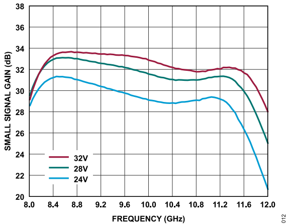
Figure 12. Small Signal Gain vs. Frequency for Various Supply Voltages, I_{DQ} = 200 \text{ mA}
