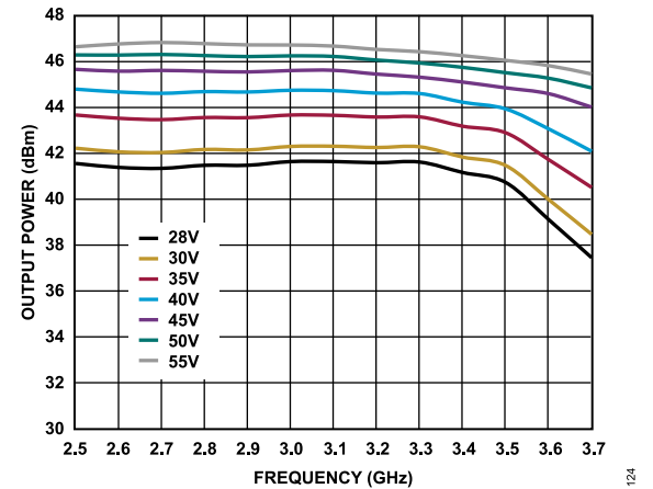
Figure 24. P_{OUT} vs. Frequency at Various Supply Voltages, P_{IN} = 21 dBm, I_{DQ} = 300 mA
