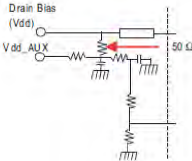
Figure 2. On-chip 50\ \Omega Resistor
