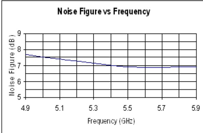
Figure 8 Noise Figure
