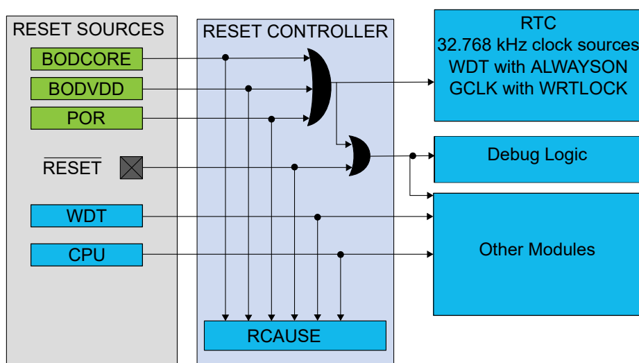
Figure 18-1. Reset System
