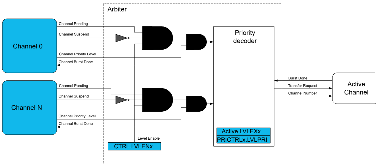
Figure 25-4. Arbiter Overview
