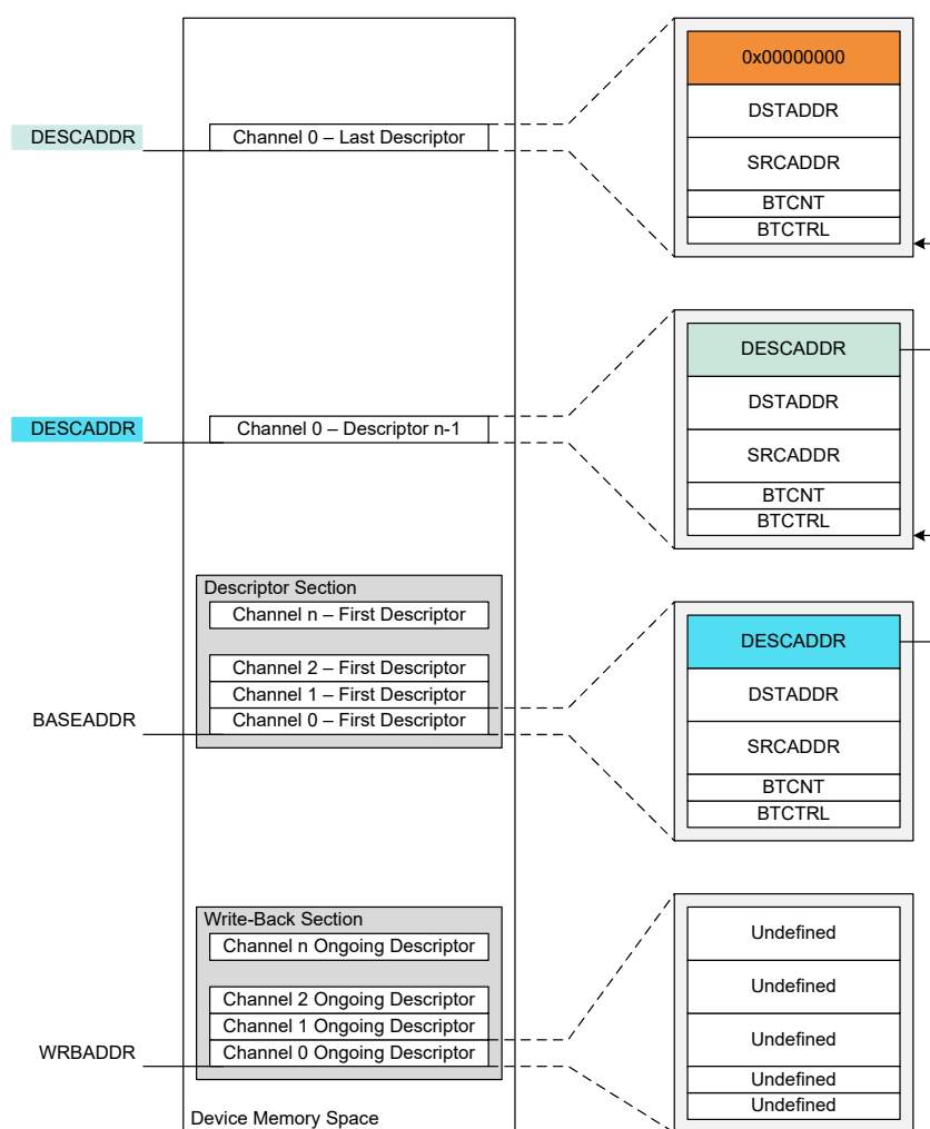
Figure 25-3. Memory Sections
