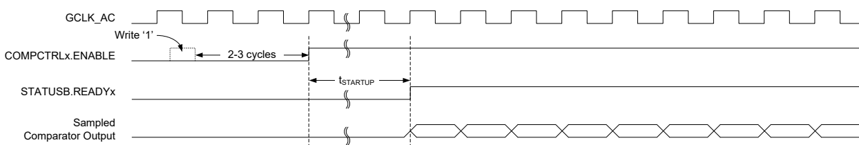
Figure 40-10. Continuous Mode SleepWalking
