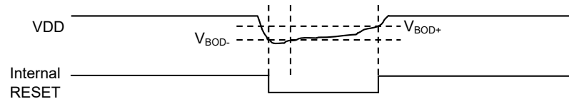
Figure 46-2. BODVDD Hysteresis ON
