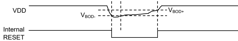
Figure 47-3. BODVDD Hysteresis ON
