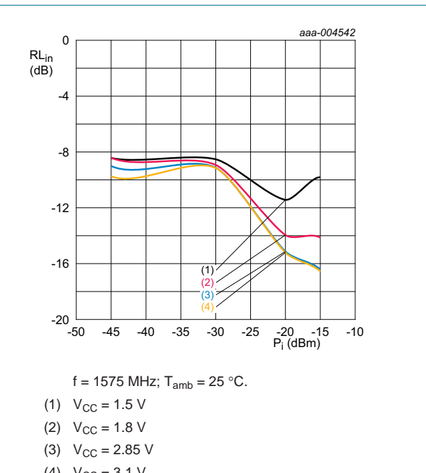
Fig 17. Input return loss as a function of input power; typical values
