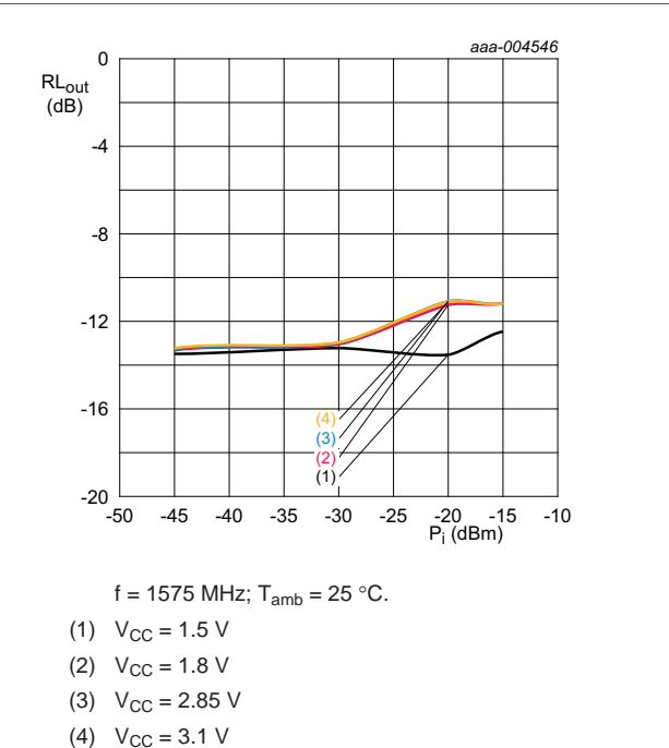
Fig 21. Output return loss as a function of input power; typical values
