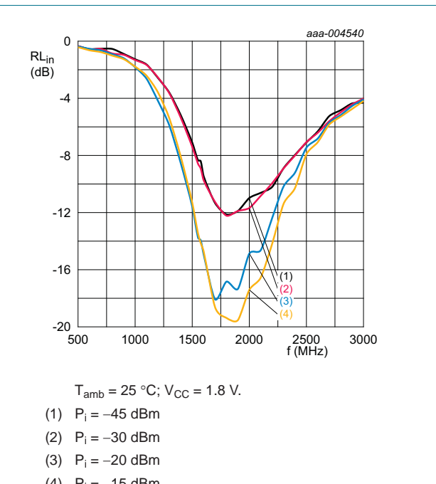
Fig 15. Input return loss as a function of frequency; typical values
