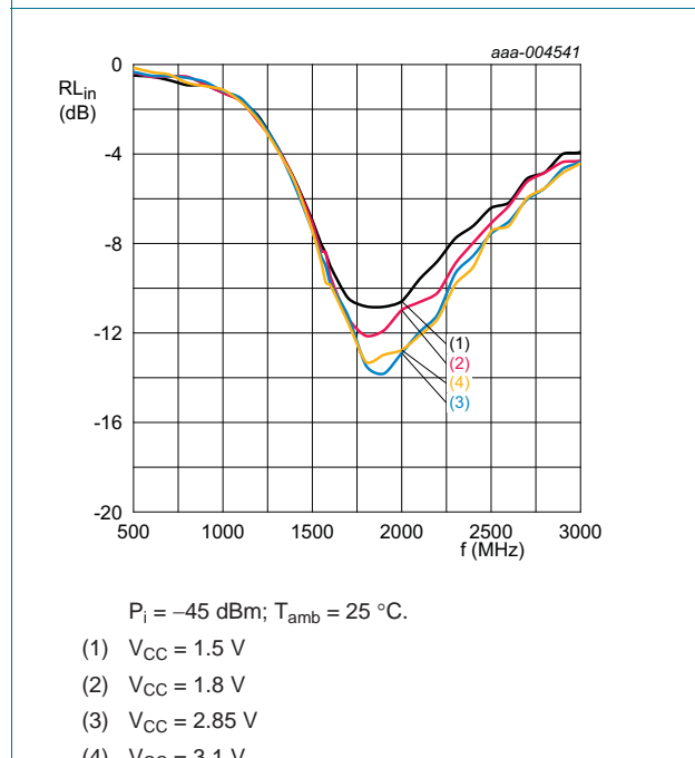
Fig 16. Input return loss as a function of frequency; typical values
