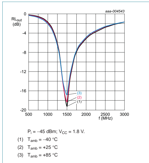
Fig 18. Output return loss as a function of frequency; typical values
