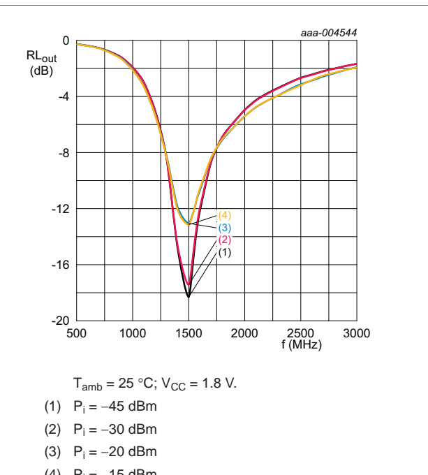
Fig 19. Output return loss as a function of frequency; typical values
