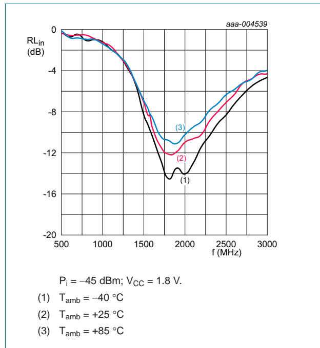
Fig 14. Input return loss as a function of frequency; typical values
