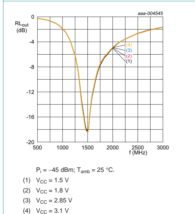
Fig 20. Output return loss as a function of frequency; typical values
