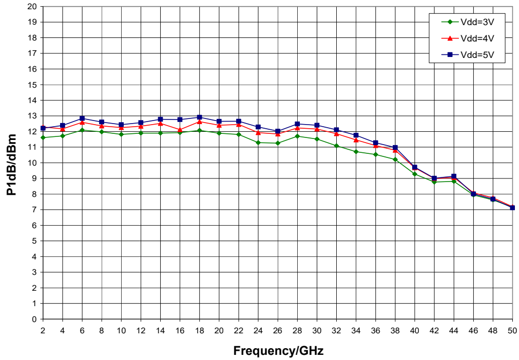
P1dB vs. V dd , I dd = 40mA, T A = 25 °C
