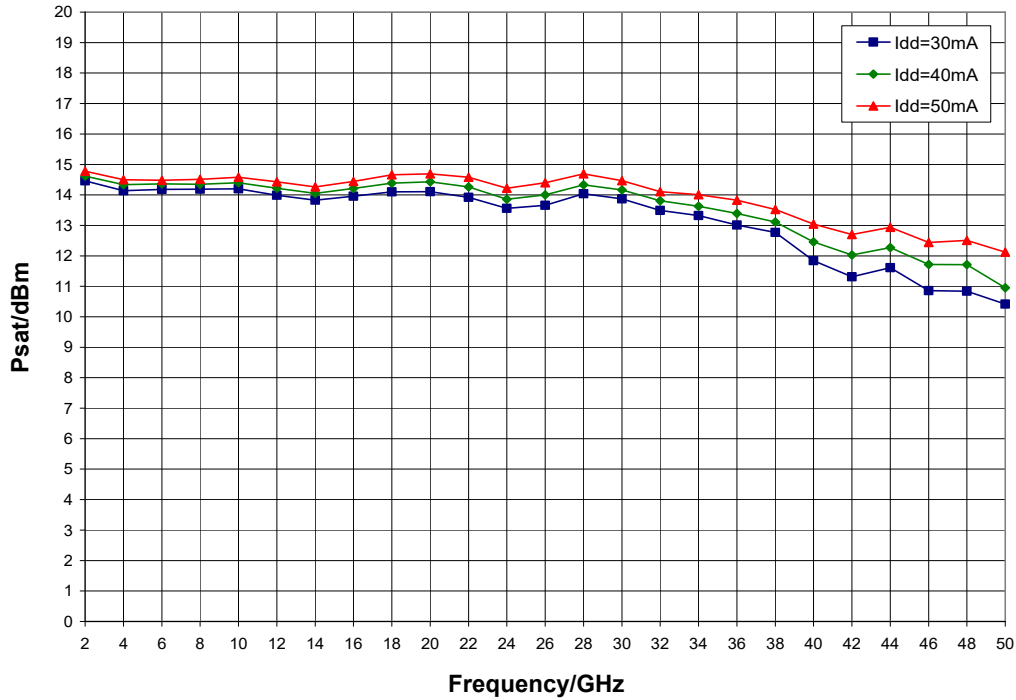
Psat vs. I dd , V dd = 3 V, T A = 25 °C
