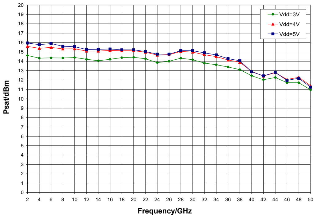
Psat vs. V_{dd} , I_{dd} = 40\text{mA} , T_A = 25\text{ }^\circ\text{C}
