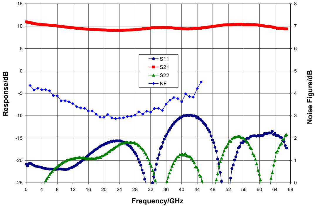
Broadband Performance, V_{dd} = 3\text{ V} , I_{dd} = 40\text{ mA} , T_A = 25\text{ }^\circ\text{C}
