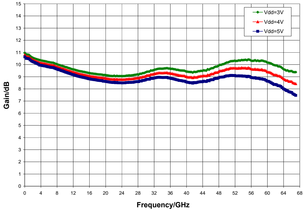
Gain vs. V_{dd} , I_{dd} = 40 \text{ mA} , T_A = 25 \text{ }^\circ\text{C}
