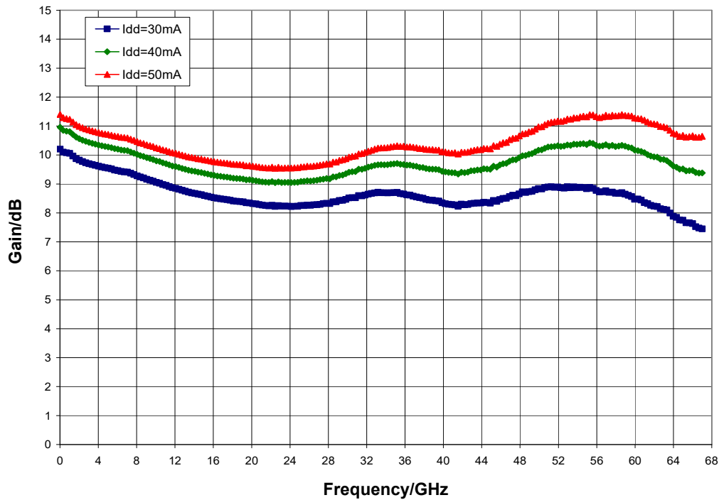
Gain vs. I_{dd} , V_{dd} = 3 \text{ V} , T_A = 25 \text{ }^\circ\text{C}
