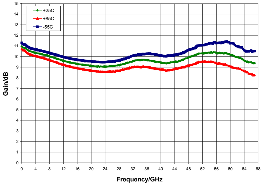
Gain vs. Temperature, V_{dd} = 3\text{ V} , T_A = 25\text{ }^\circ\text{C}
