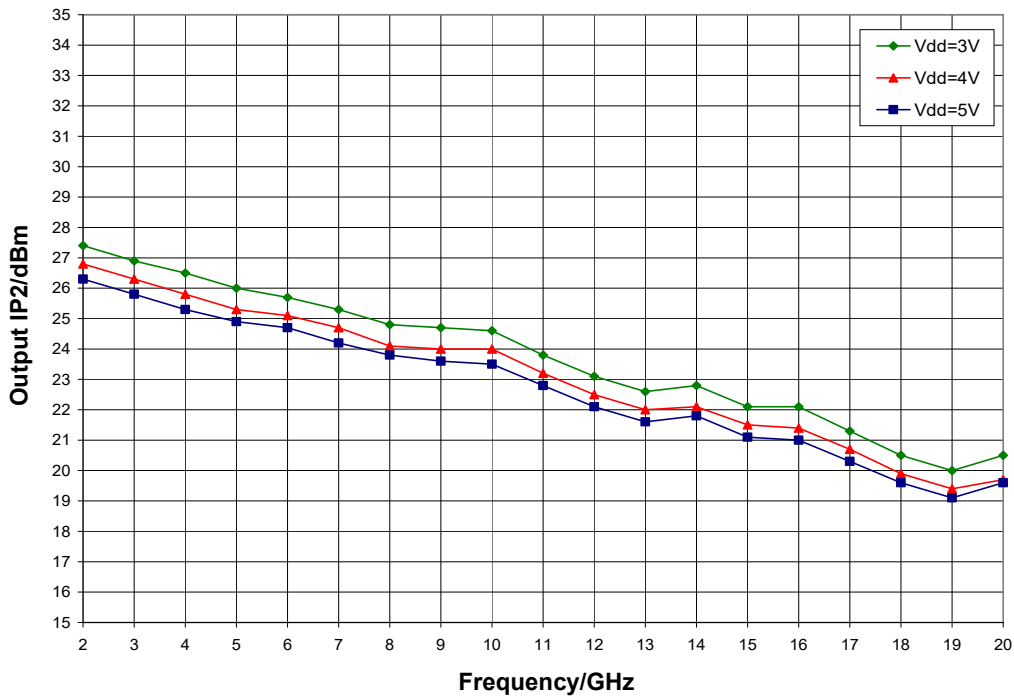
Output IP2 vs. V_{dd} , I_{dd} = 40\text{mA} , T_A = 25\text{ }^\circ\text{C}
