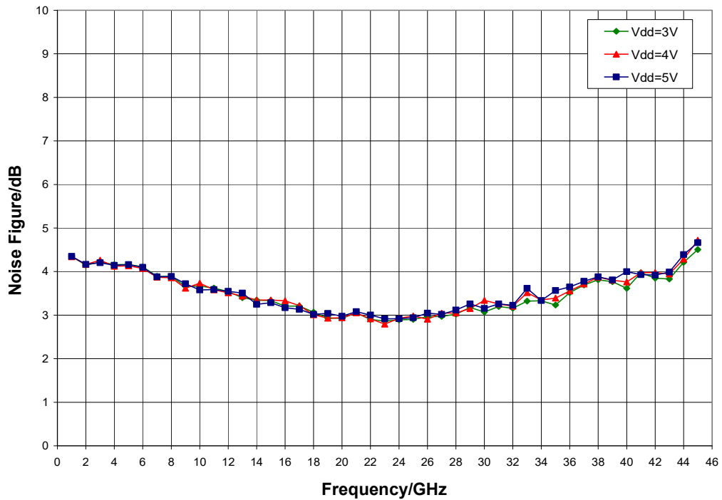
Noise Figure vs. V_{dd} , I_{dd} = 40\text{ mA} , T_A = 25\text{ }^\circ\text{C}
