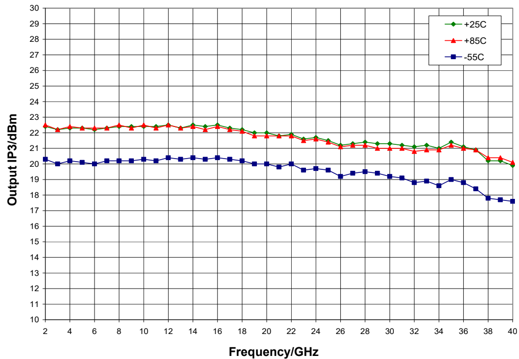
Output IP3 vs. Temperature, V dd = 3 V
