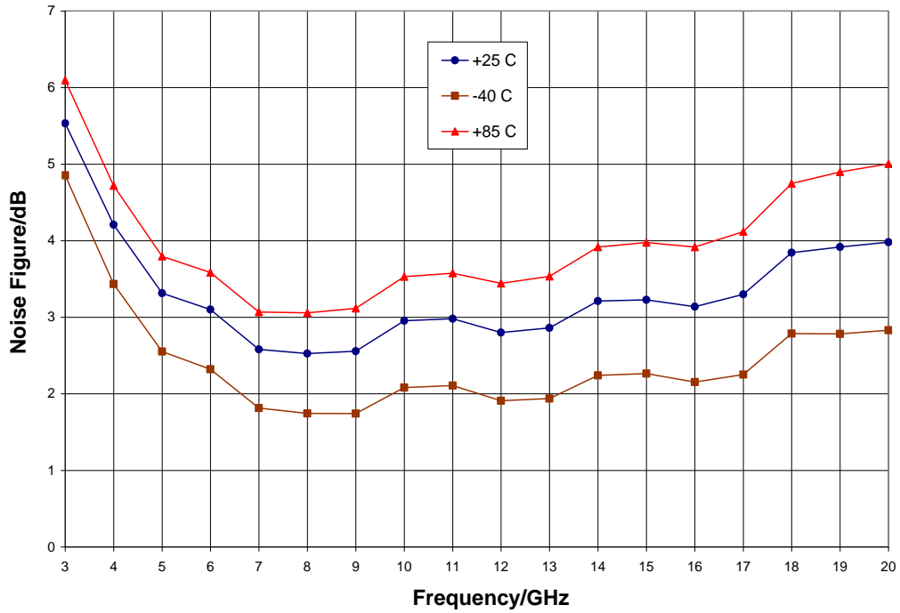
Noise Figure vs. Temperature, V_{dd} = 10\text{ V} , V_{gg} = -0.55\text{ V}
