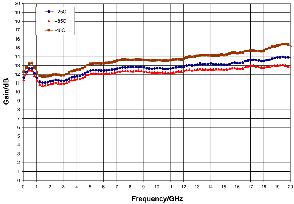
Gain vs. Temperature, V_{dd} = 10\text{ V} , V_{gg} = -0.55\text{ V}
