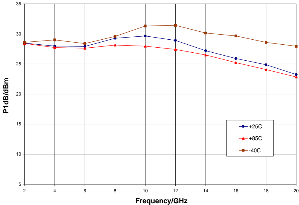
P1dB vs. Temperature, V_{dd} = 10\text{ V} , V_{gg} = -0.55\text{ V}
