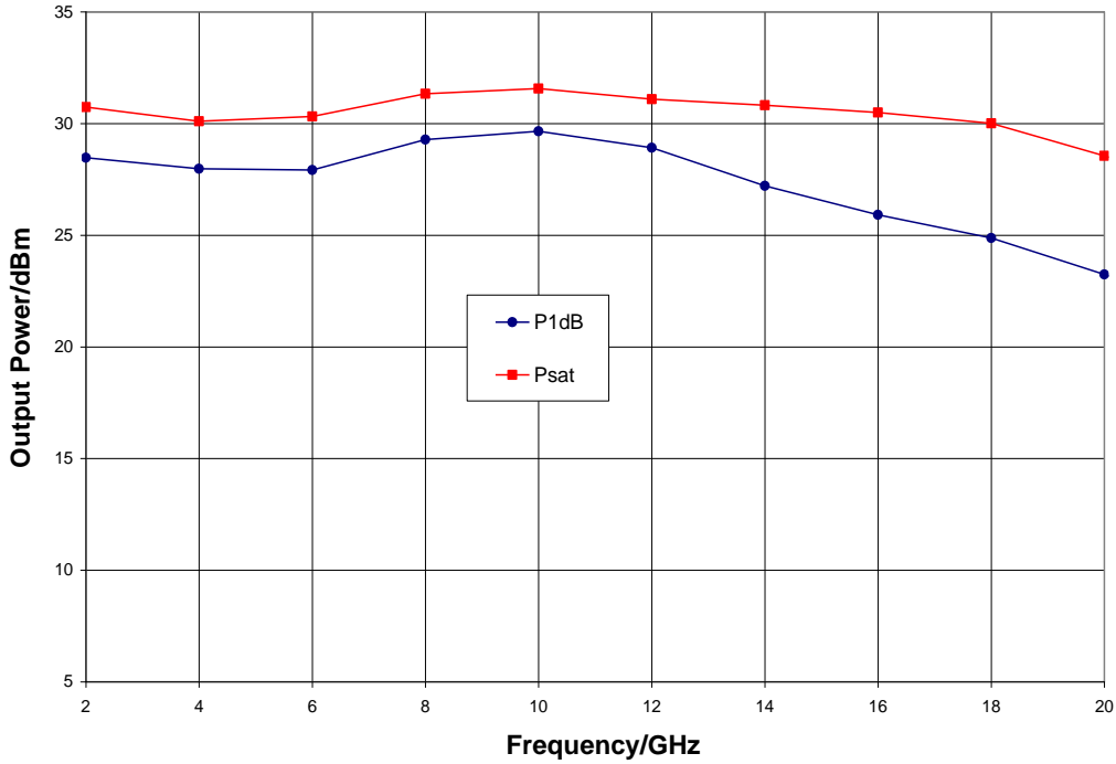
Output Power, V_{dd} = 10\text{ V} , V_{gg} = -0.55\text{ V} , T_A = 25^\circ\text{ C}
