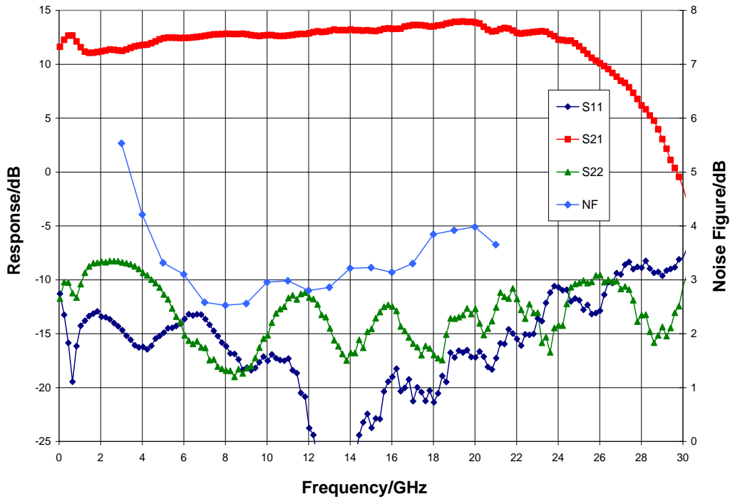
Broadband Performance, V_{dd} = 10\text{ V} , V_{gg} = -0.55\text{ V} , I_{dd} = 380\text{ mA} , T_A = 25^\circ\text{ C}
