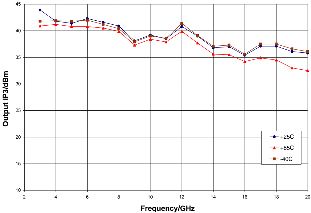
Output IP3 vs. Temperature, V_{dd} = 10\text{ V} , V_{gg} = -0.55\text{ V}
