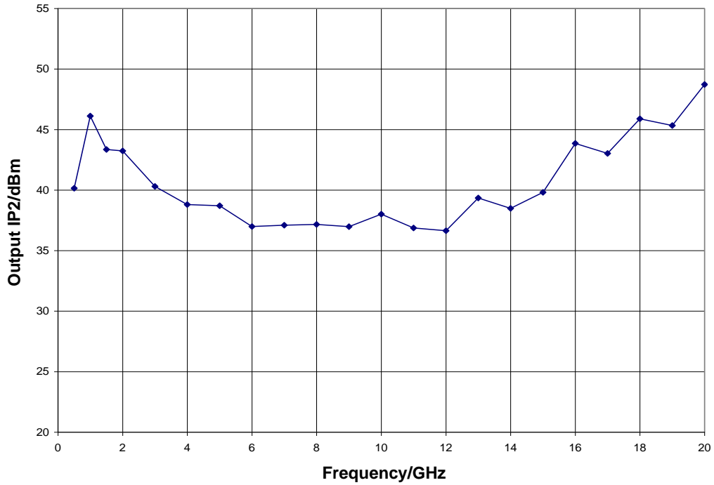
Output IP2, V_{dd} = 10\text{ V} , V_{gg} = -0.55\text{ V}
