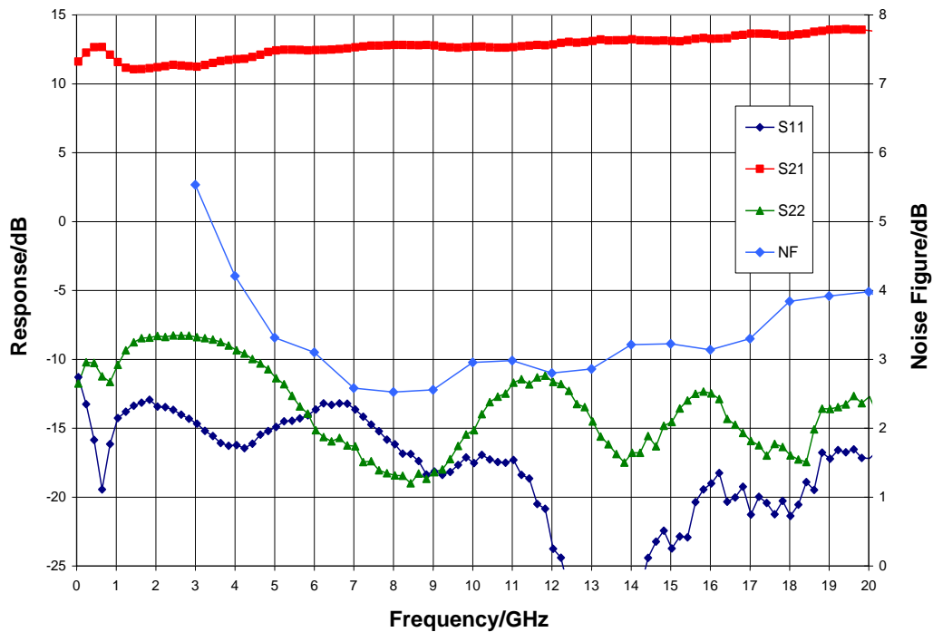
Narrow-band Performance, V_{dd} = 10\text{ V} , V_{gg} = -0.55\text{ V} , I_{dd} = 380\text{ mA} , T = 25^\circ\text{ C}
