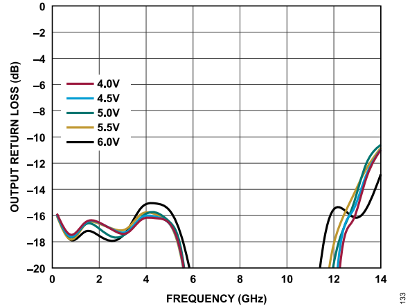
Figure 33. Output Return Loss vs. Frequency for Various Supply Voltages, 200MHz to 14GHz, I_{DQ} = 110mA
