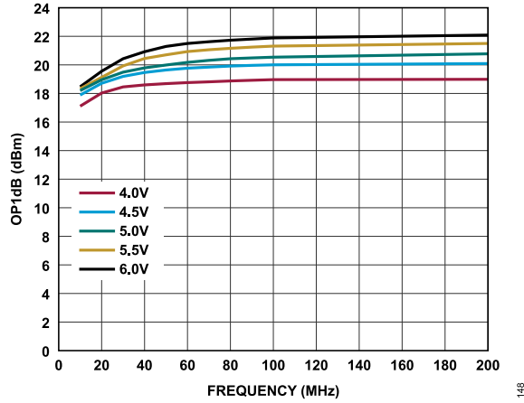
Figure 48. OP1dB vs. Frequency for Various Supply Voltages, 10MHz to 200MHz, I_{DQ} = 110mA
