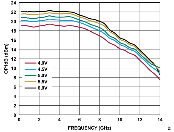
Figure 51. OP1dB vs. Frequency for Various Supply Voltages, 200MHz to 14GHz, V_{DD} = 5V , I_{DQ} = 110mA
