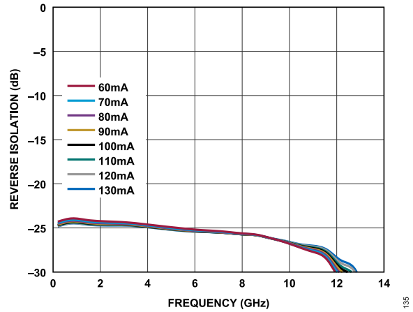
Figure 35. Reverse Isolation vs. Frequency for Various I_{DQ} Values, 200MHz to 14GHz, V_{DD} = 5V
