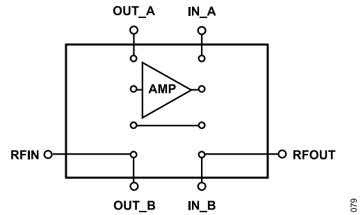
Figure 119. External Bypass B Mode, VA = 3.3V and VB = 0V
