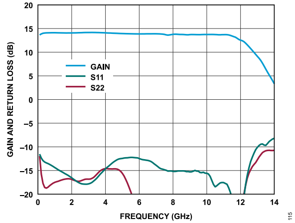
Figure 15. Gain and Return Loss vs. Frequency, 200MHz to 14GHz, V_{DD} = 5V , I_{DQ} = 110mA
