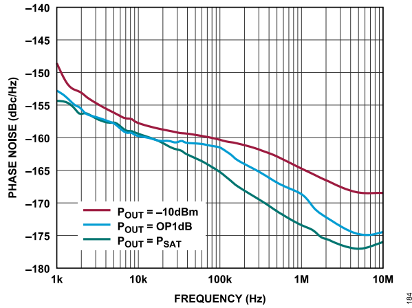
Figure 84. Phase Noise vs. Frequency at 5GHz for Various P_{OUT} Values, V_{DD} = 5V, I_{DQ} = 110mA
