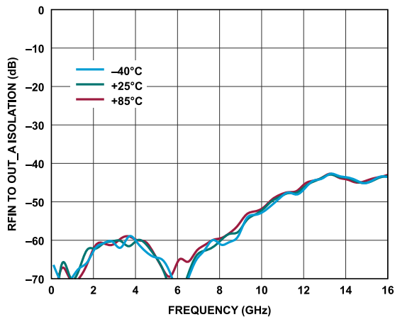
Figure 88. RFIN to OUT_A Isolation vs. Frequency for Various Temperatures, 10MHz to 16GHz
