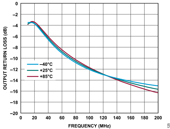
Figure 25. Output Return Loss vs. Frequency for Various Temperatures, 10MHz to 200MHz, V_{DD} = 5V , I_{DQ} = 110mA
