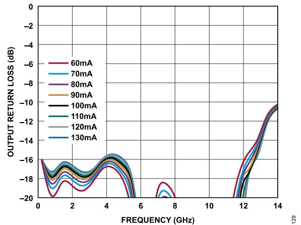
Figure 29. Output Return Loss vs. Frequency for Various I_{DQ} Values, 200MHz to 14GHz, V_{DD} = 5V
