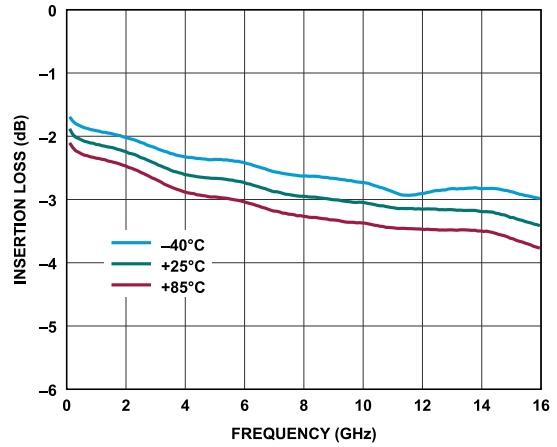
Figure 89. Insertion Loss vs. Frequency for Various Temperatures, 10MHz to 16GHz
