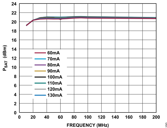
Figure 50. P_{SAT} vs. Frequency for Various I_{DQ} Values, 10MHz to 200MHz, V_{DD} = 5V
