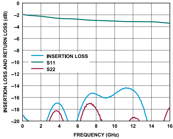
Figure 86. Insertion Loss and Return Loss vs. Frequency, 10MHz to 16GHz
