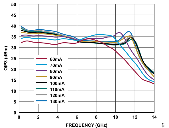
Figure 71. OIP3 vs. Frequency for Various I_{DQ} Values, 200MHz to 14GHz, V_{DD} = 5V
