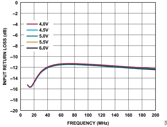
Figure 24. Input Return Loss vs. Frequency for Various Supply Voltages, 10MHz to 200MHz, I_{DQ} = 110mA
