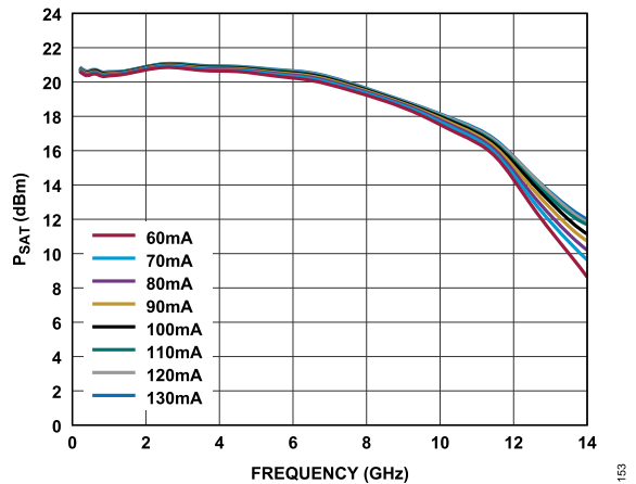
Figure 53. P_{SAT} vs. Frequency for Various I_{DQ} Values, 200MHz to 14GHz, V_{DD} = 5V
