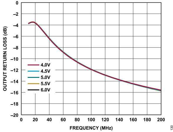
Figure 30. Output Return Loss vs. Frequency for Various Supply Voltages, 10MHz to 200MHz, I_{DQ} = 110mA
