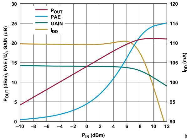
Figure 61. P_{OUT} , PAE, Gain, and I_{DD} vs. P_{IN} , Power Compression at 2GHz, V_{DD} = 5V
