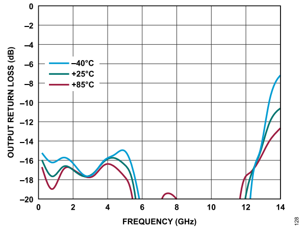
Figure 28. Output Return Loss vs. Frequency for Various Temperatures, 200MHz to 14GHz, V_{DD} = 5V , I_{DQ} = 110mA
