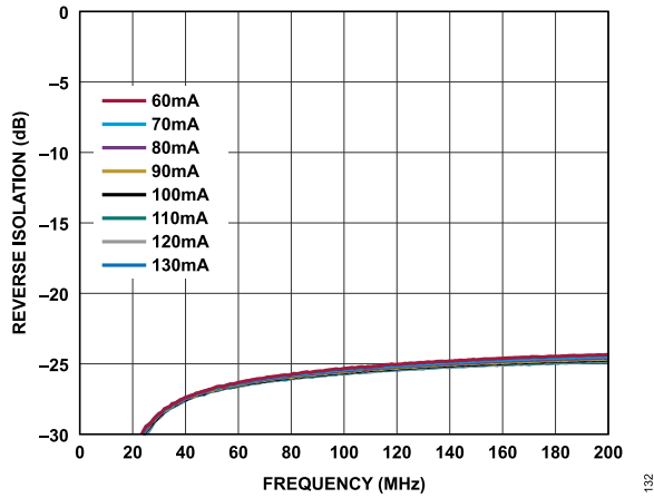
Figure 32. Reverse Isolation vs. Frequency for Various I_{DQ} Values, 10MHz to 200MHz, V_{DD} = 5V
