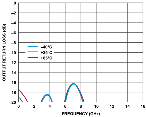
Figure 90. Output Return Loss vs. Frequency for Various Temperatures, 10MHz to 16GHz
