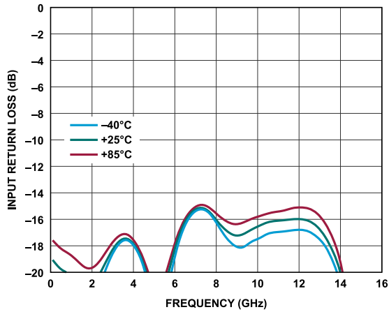
Figure 87. Input Return Loss vs. Frequency for Various Temperatures, 10MHz to 16GHz
