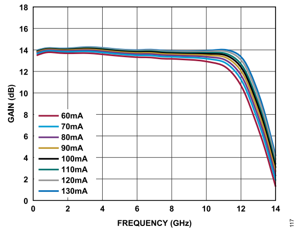
Figure 17. Gain vs. Frequency for Various I_{DQ} Values, V_{DD} = 5V , I_{DQ} = 110mA
