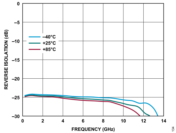
Figure 34. Reverse Isolation vs. Frequency for Various Temperatures, 200MHz to 14GHz, V_{DD} = 5V , I_{DQ} = 110mA
