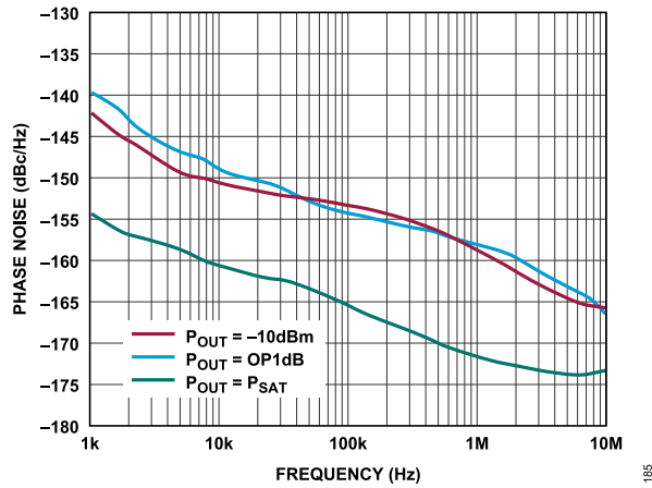
Figure 85. Phase Noise vs. Frequency at 10GHz for Various P_{OUT} Values, V_{DD} = 5V, I_{DQ} = 110mA
