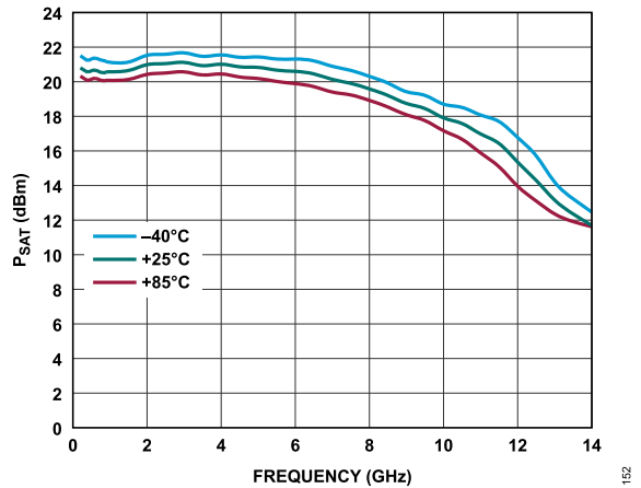
Figure 52. P_{SAT} vs. Frequency for Various Temperatures, 200MHz to 14GHz, V_{DD} = 5V , I_{DQ} = 110mA
