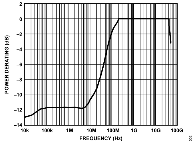
Figure 2. RF Input Power Derating Curve
