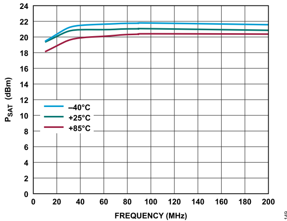
Figure 49. Saturated Power ( P_{SAT} ) vs. Frequency for Various Temperatures, 10MHz to 200MHz, V_{DD} = 5V , I_{DQ} = 110mA
