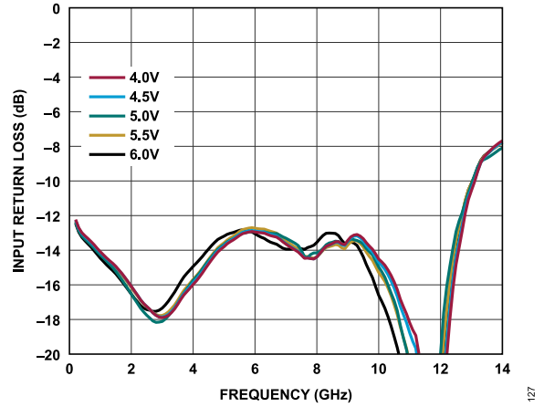
Figure 27. Input Return Loss vs. Frequency for Various Supply Voltages, 200MHz to 14GHz, I_{DQ} = 110mA
