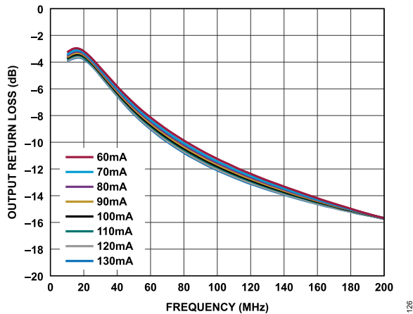
Figure 26. Output Return Loss vs. Frequency for Various I_{DQ} Values, 10MHz to 200MHz, V_{DD} = 5V
