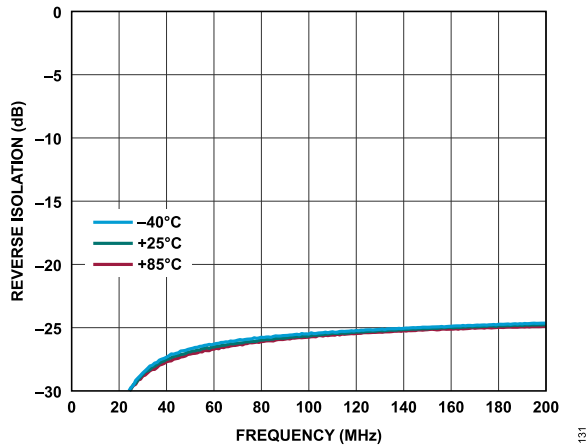
Figure 31. Reverse Isolation vs. Frequency for Various Temperatures, 10MHz to 200MHz, V_{DD} = 5V , I_{DQ} = 110mA
