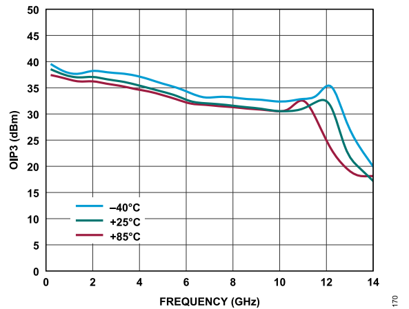
Figure 70. OIP3 vs. Frequency for Various Temperatures, 200MHz to 14GHz, V_{DD} = 5V , I_{DQ} = 110mA
