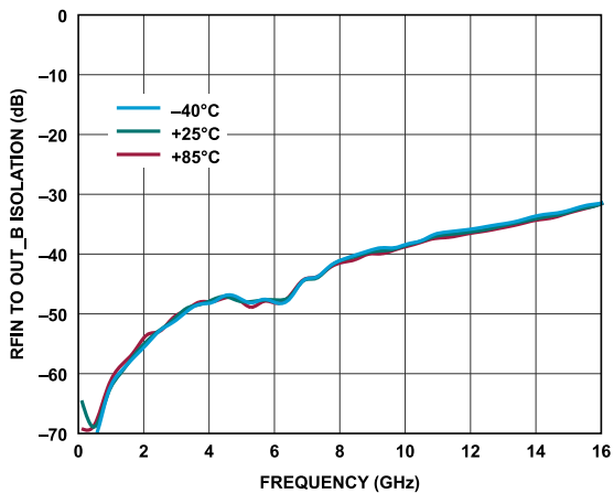
Figure 91. RFIN to OUT_B Isolation vs. Frequency for Various Temperatures, 10MHz to 16GHz
