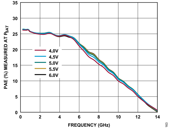
Figure 63. PAE Measured at P_{SAT} vs. Frequency for Various Supply Voltages, 200MHz to 14GHz, I_{DQ} = 110mA
