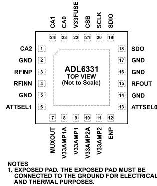
Figure 6. Pin Configuration
