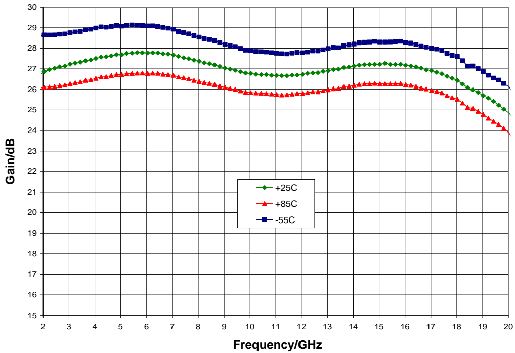
Gain vs. Temperature, V_{dd} = 3.0\text{ V} , V_{gg} = 2.0\text{ V}
