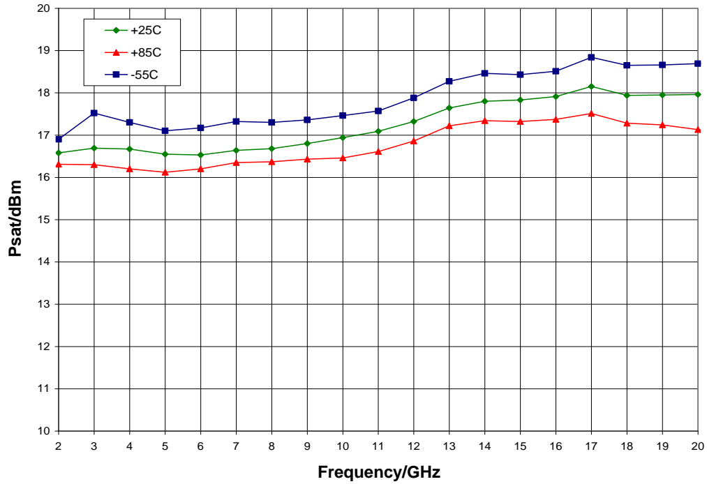
Psat vs. Temperature, V_{dd} = 3.0\text{ V} , V_{gg} = 2.0\text{ V}
