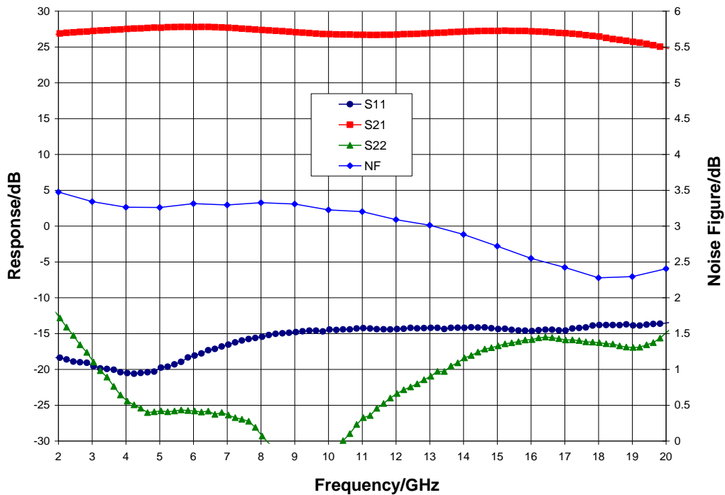
Narrow-band Performance, V_{dd} = 3.0\text{ V} , V_{gg} = 2.0\text{ V} , I_{dd} = 145\text{ mA} , T_A = 25\text{ °C}
