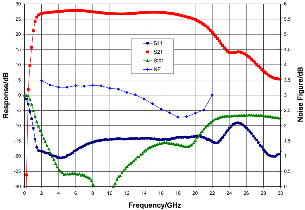
Broadband Performance, V_{dd} = 3.0\text{ V} , V_{gg} = 2.0\text{ V} , I_{dd} = 145\text{ mA} , T_A = 25\text{ °C}
