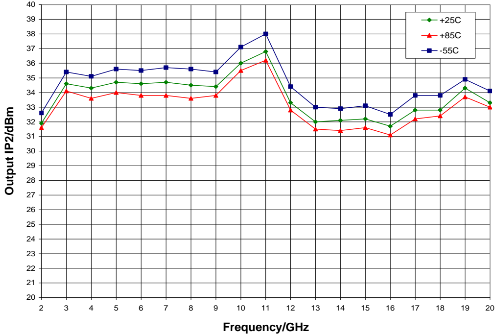
Output IP2 vs. Temperature, V_{dd} = 3.0\text{ V} , V_{gg} = 2.0\text{ V}
