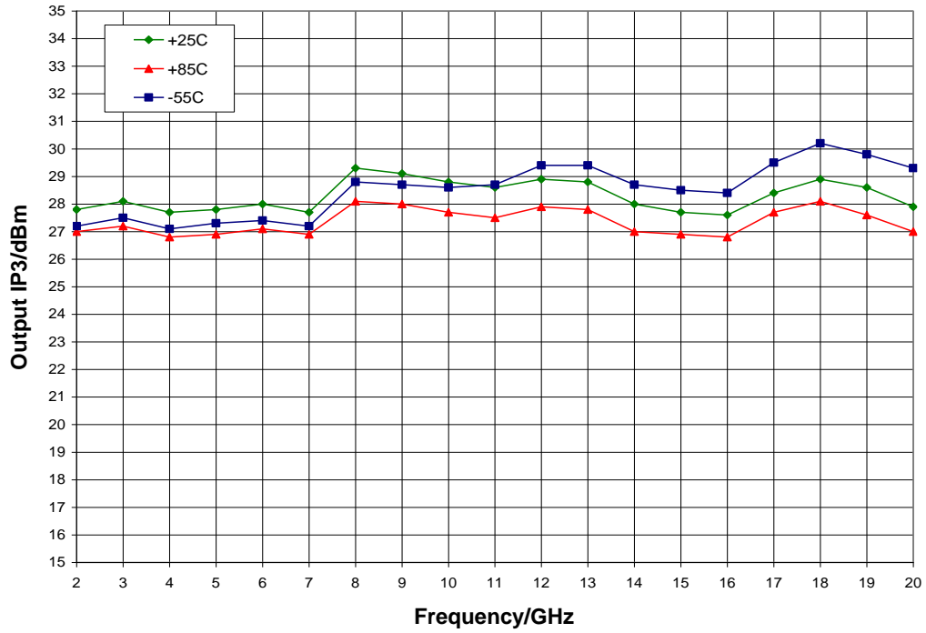
Output IP3 vs. Temperature, V_{dd} = 3.0\text{ V} , V_{gg} = 2.0\text{ V}
