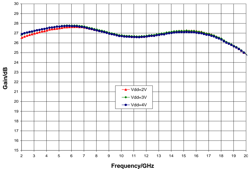
Gain vs. V_{dd} , V_{gg} = 2.0\text{ V} , T_A = 25\text{ }^\circ\text{C}
