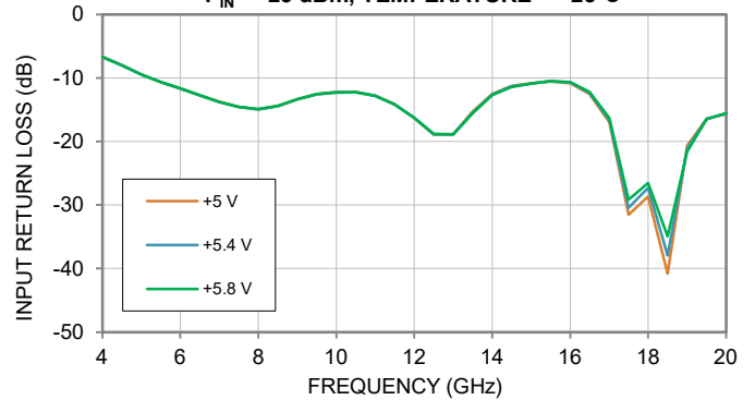
INPUT RETURN LOSS vs. BASE VOLTAGE ( V_B ) P_{IN} = -25 dBm, TEMPERATURE = +25°C
