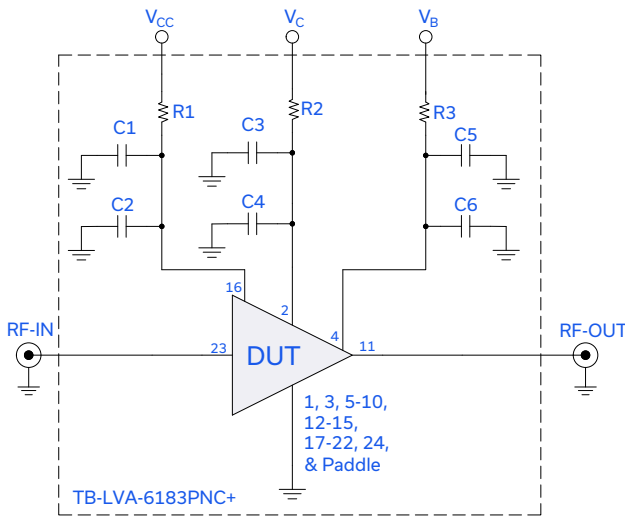
Figure 2. LVA-6183PN+ Characterization and Application Circuit
