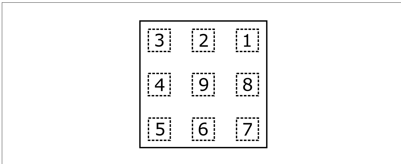
Figure 1: BGA10H1MN9 Pin Configuration (top view)
