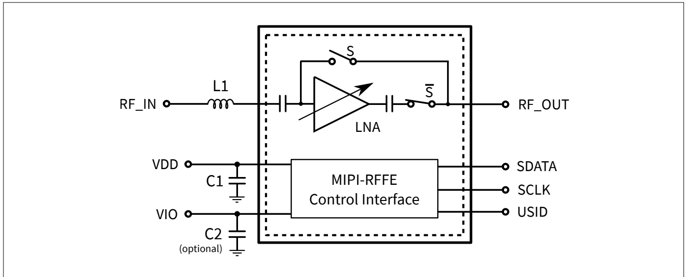
Figure 2: BGA10H1MN9 Application Schematic
