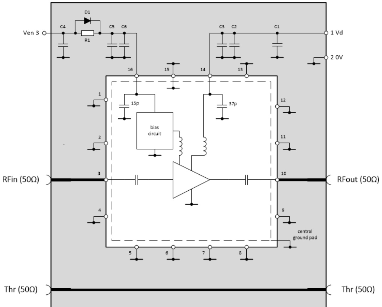
Figure 31: EV90G302 Schematic
