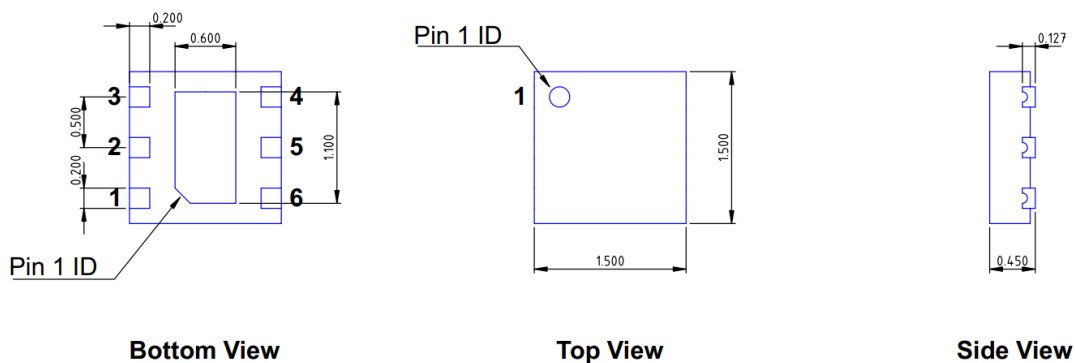
DFN6 1.5x1.5mm Dimensions in millimeters Dimensional Tolerance: \pm 0.05
