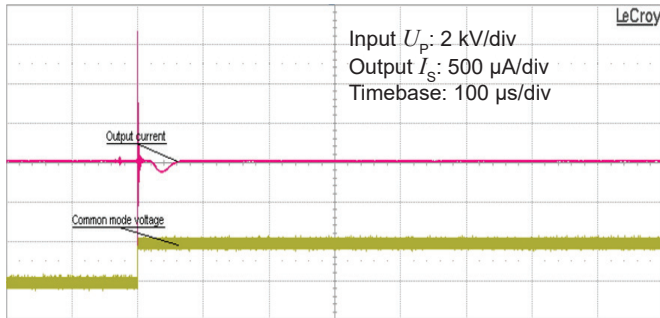
Figure 13: Typical common mode perturbation (2000 V step with 6 kV/μs, R_M = 100 \Omega )
