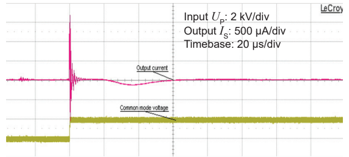
Figure 14: Detail of typical common mode perturbation (2000 V step with 6 kV/μs, R_M = 100 \Omega )
