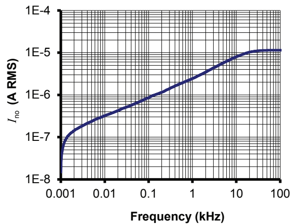
Figure 15: Typical total output RMS noise current with R_M = 50 \Omega ( f_c is upper cut-off frequency of bandpass, low cut off frequency is 1 Hz)
