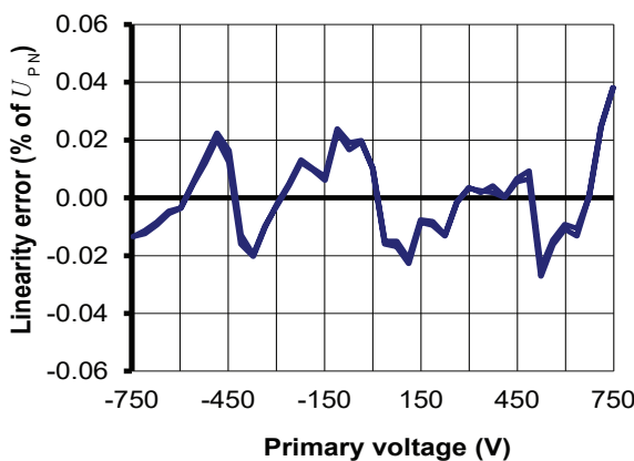
Figure 16: Typical linearity error at 25 °C
