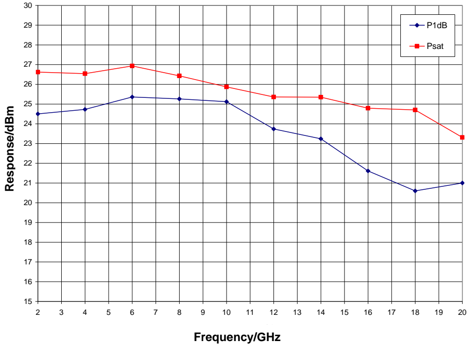
Output Power, V_{dd} = 8.0\text{ V} , V_{gg} = -1.0\text{ V} , T_A = 25\text{ °C}
