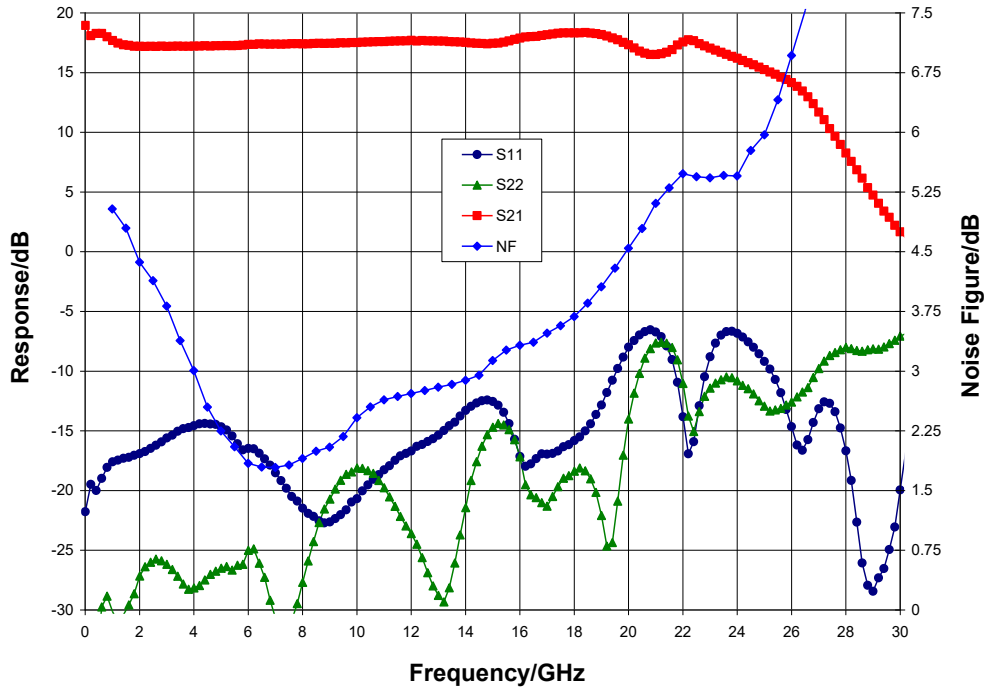
Broadband Performance, V_{dd} = 8.0\text{ V} , V_{gg} = -1.0\text{ V} , T_A = 25\text{ }^\circ\text{C}
