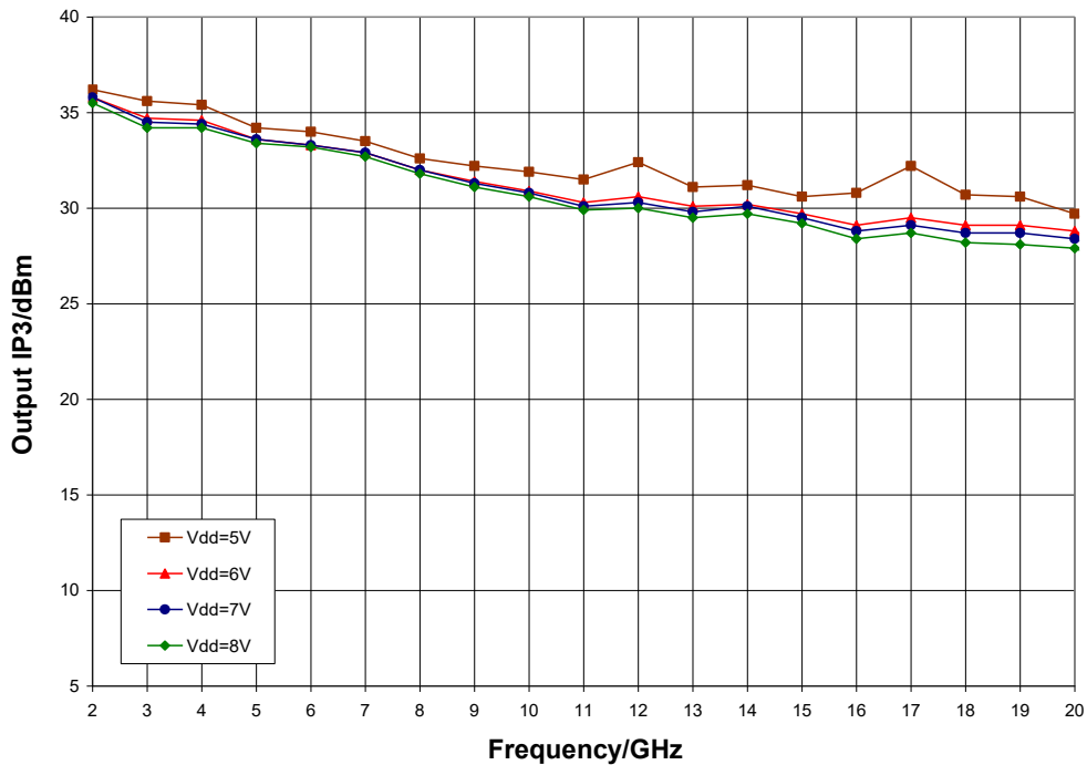
Output IP3 vs. V_{dd} , T_A = 25\text{ }^\circ\text{C}
