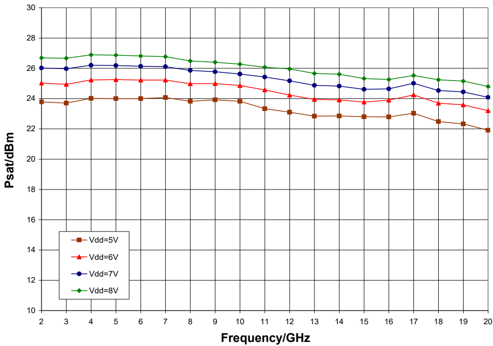
Psat vs. V_{dd} , T_A = 25\text{ }^\circ\text{C}
