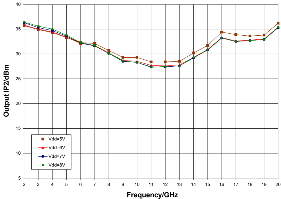
Output IP2 vs. V_{dd} , T_A = 25\text{ }^\circ\text{C}
