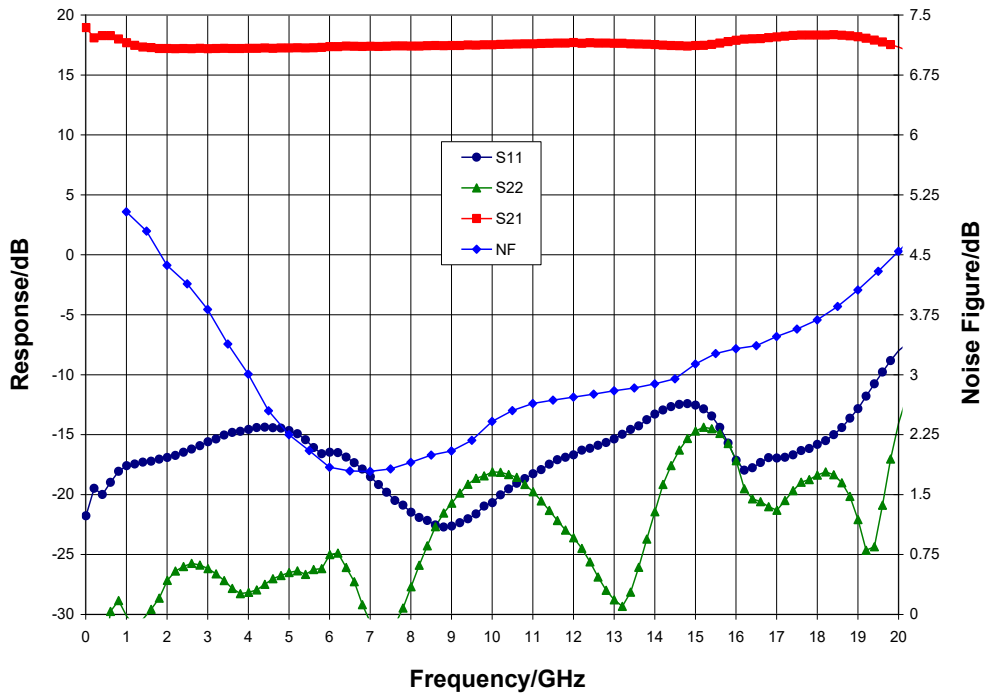
Narrow-band Performance, V_{dd} = 8.0\text{ V} , V_{gg} = -1.0\text{ V} , T_A = 25\text{ }^\circ\text{C}
