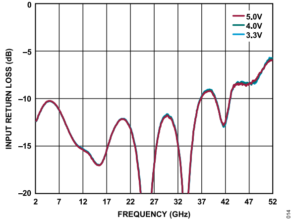
Figure 14. Input Return Loss vs. Frequency at Various V_{DD} Voltages, I_{DQ} = 85 mA, V_{GG2} = 1 V
