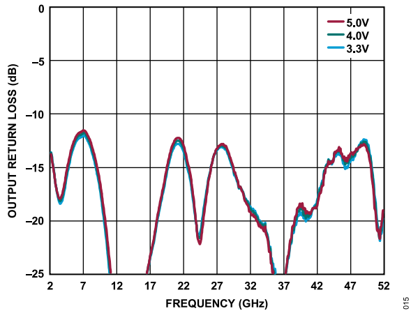
Figure 15. Output Return Loss vs. Frequency at Various V_{DD} Voltages, I_{DQ} = 85 mA, V_{GG2} = 1 V
