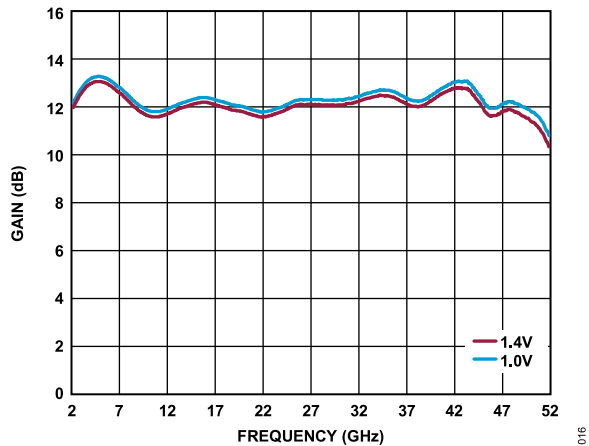
Figure 16. Gain vs. Frequency at Various V_{GG2} Voltages, V_{DD} = 5 V, I_{DQ} = 85 mA
