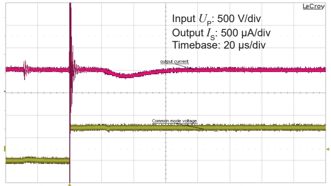
Figure 14: Detail of typical common mode perturbation (750 V step with 6 kV/μs, R_M = 100 \Omega )
