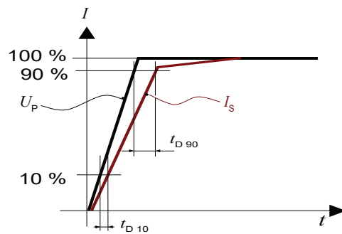
Figure 19: Delay time t_{D90} @ 90 and delay time t_{D10} @ 10
