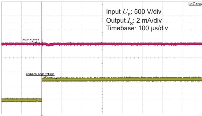
Figure 13: Typical common mode perturbation (750 V step with 6 kV/μs, R_M = 100 \Omega )
