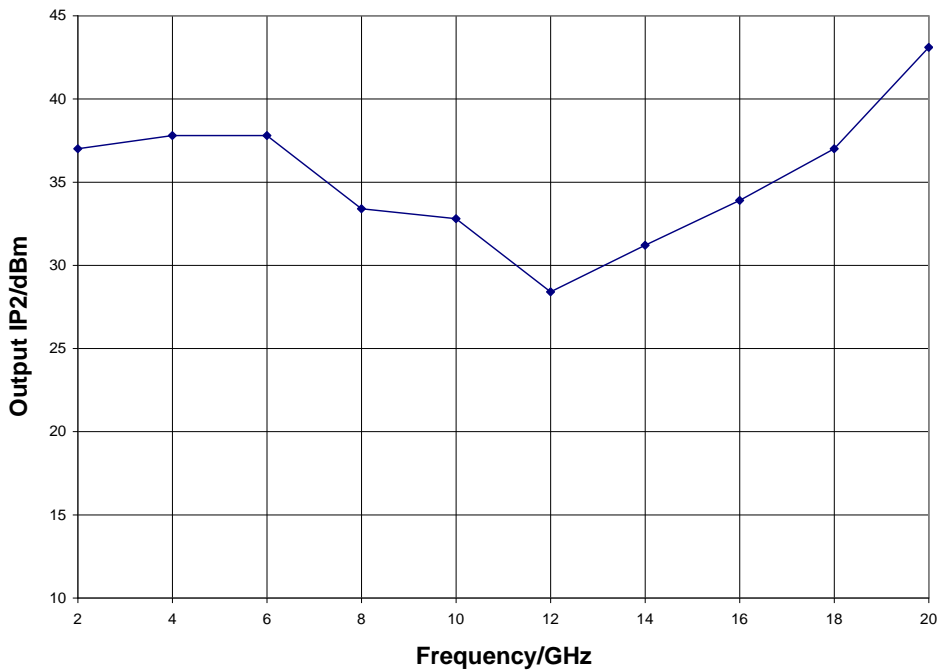
Output IP2, V_{dd} = 5.0\text{ V} , T_A = 25\text{ }^\circ\text{C}
