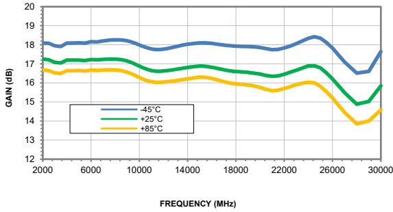
GAIN vs. FREQUENCY & TEMPERATURE @ VDD = +5.00V
